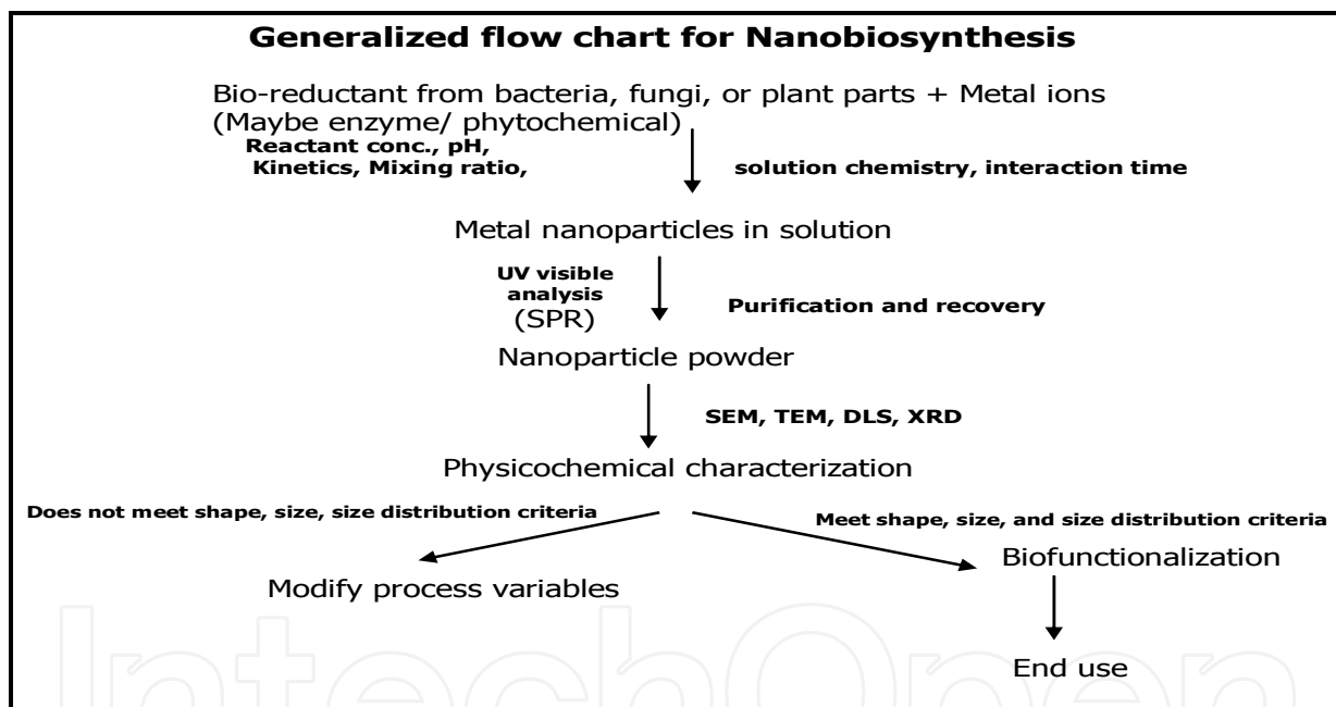
Fig. 1. Flowchart denoting the biosynthesis of nanoparticles
