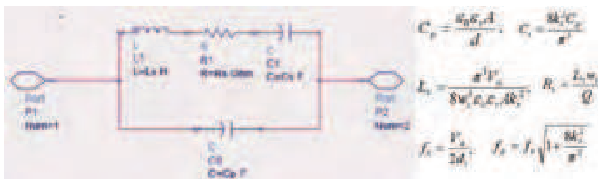
Fig. 8. FBAR resonator – BVD model.
