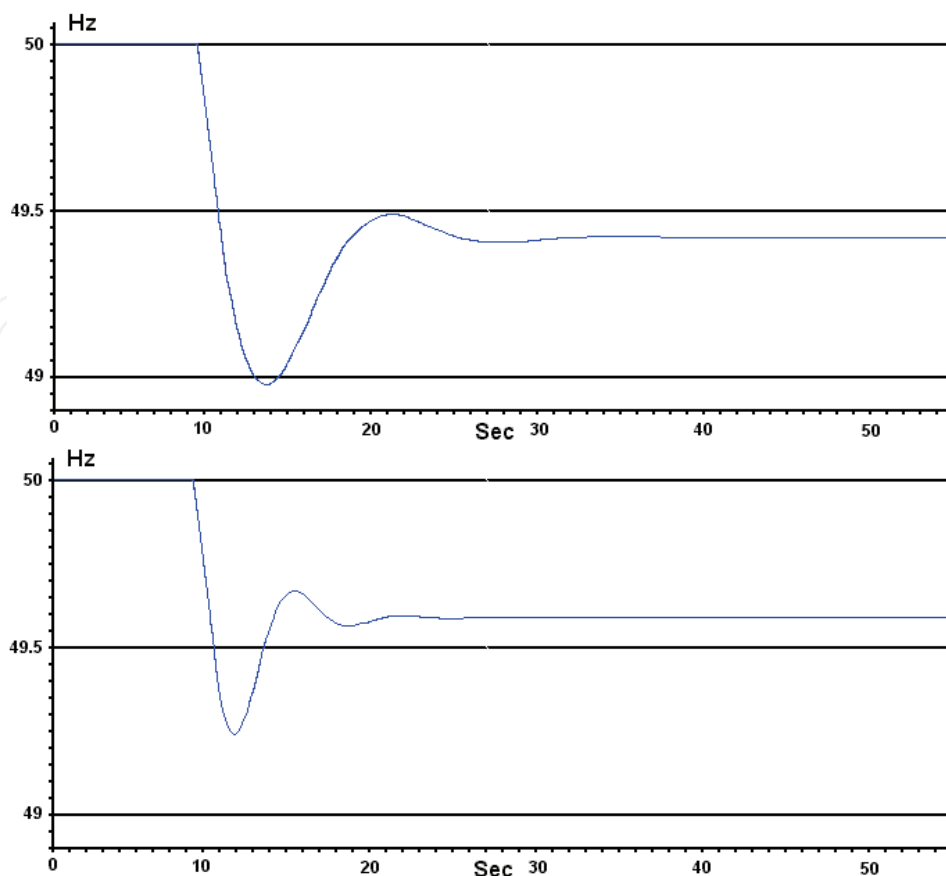
Fig. 20. Effect of dispatch on system frequency deviation
