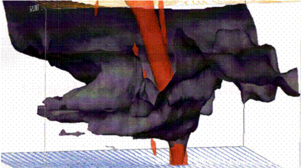
Fig. 3. Computer simulation of tornadogenesis.
