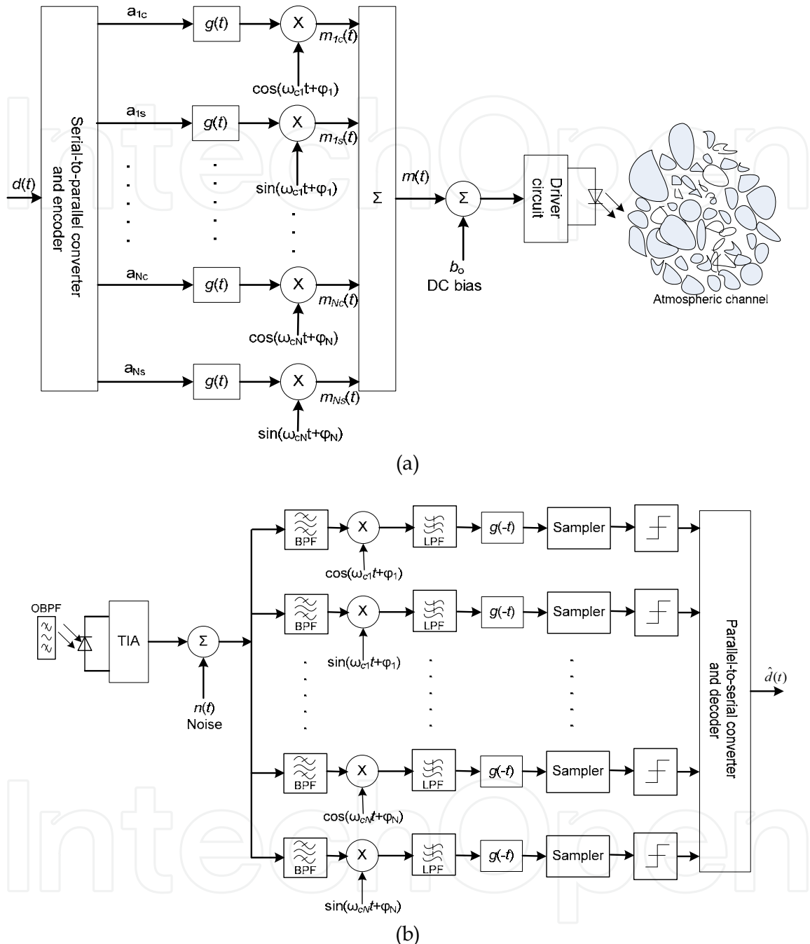
Fig. 16. Block diagram of SIM: (a) transmitter, and (b) receiver. TIA- trans-impedance
