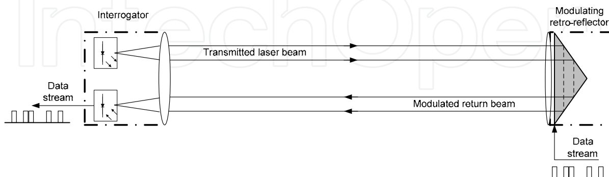
Fig. 2. Modulated retro-reflector based FSO system block diagram
