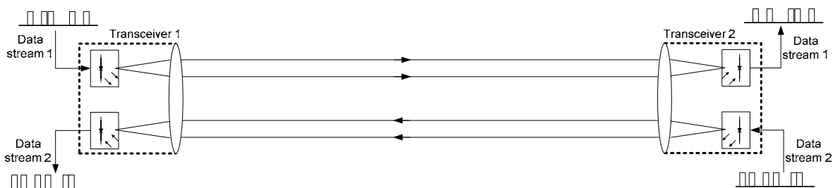
Fig. 1. Conventional FOS system block diagram
