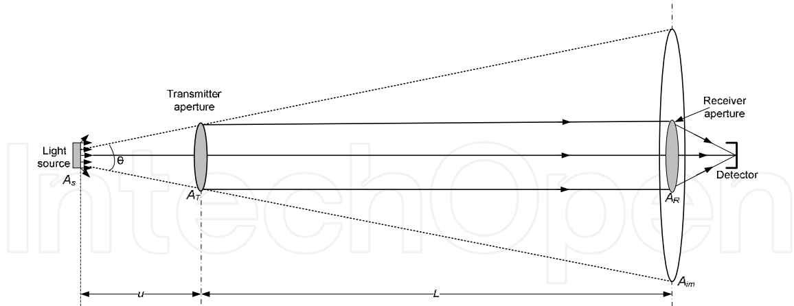
Fig. 7. Beam divergence
