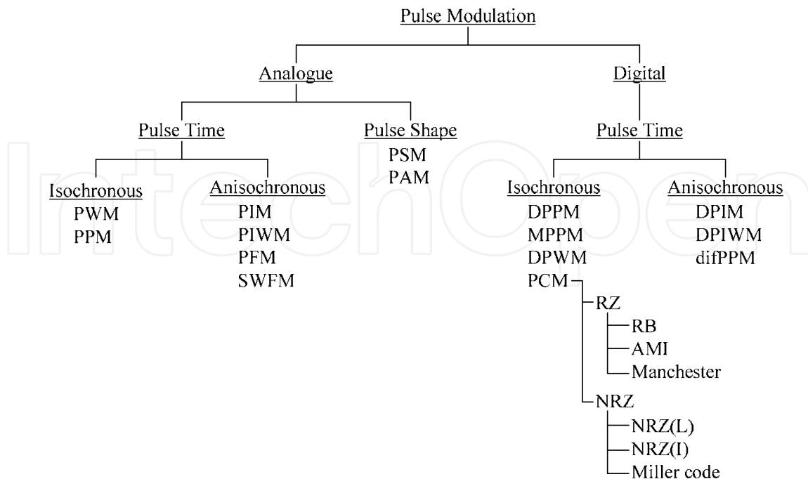
Fig. 10. Pulse modulation tree.
