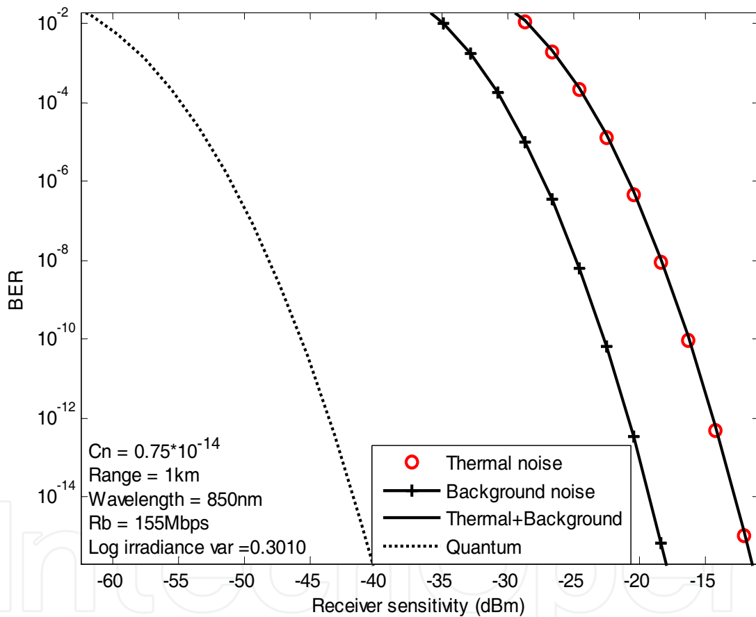
Fig. 17. The BER against the receiver sensitivity under different noise sources, with R_b = 155 Mbps, \sigma_r^2 = 0.3 and \xi = 1 .
