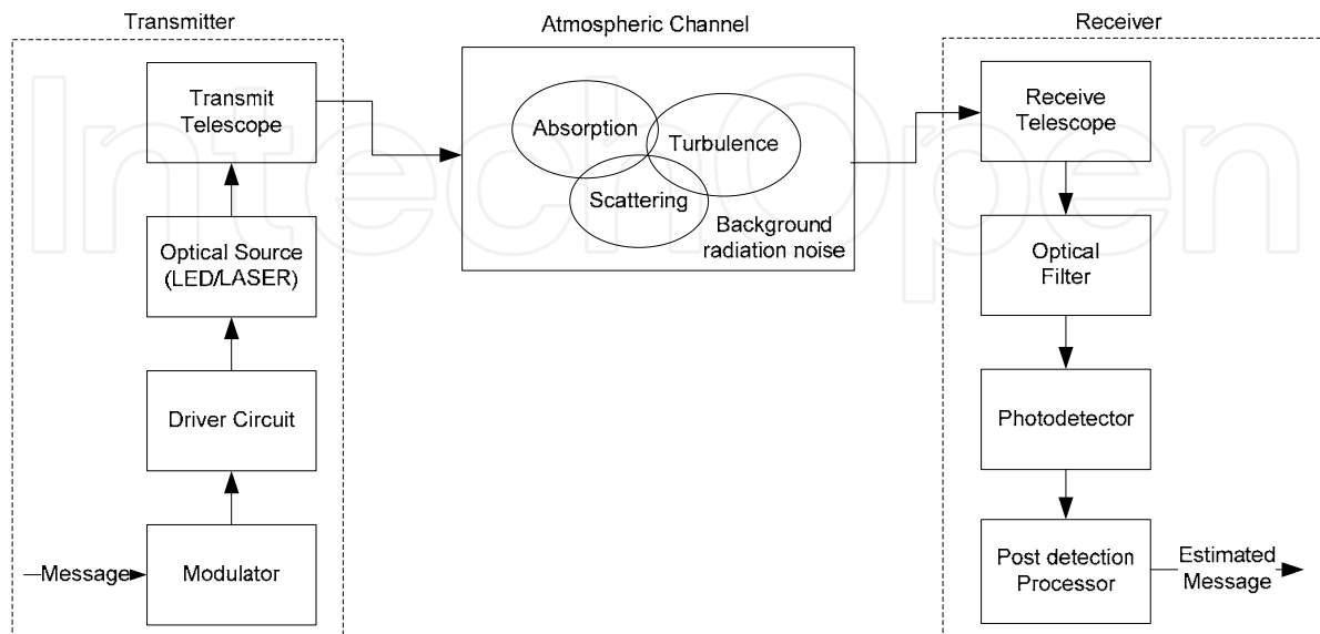
Fig. 3. Block diagram of a terrestrial FSO link
