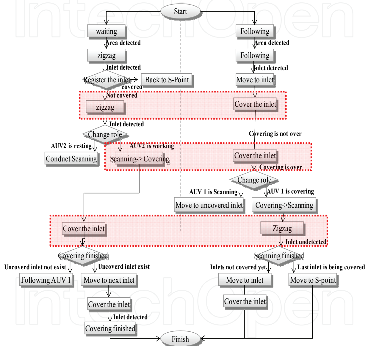
Figure 16. Simulated Multi-AUV work flow
