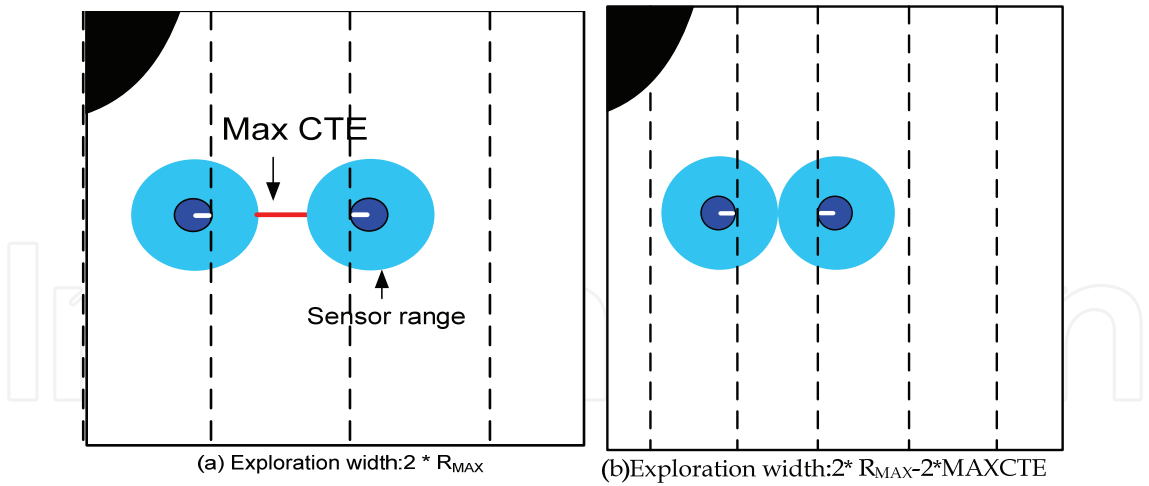
Figure 12. Calculating of EEW using CTE
