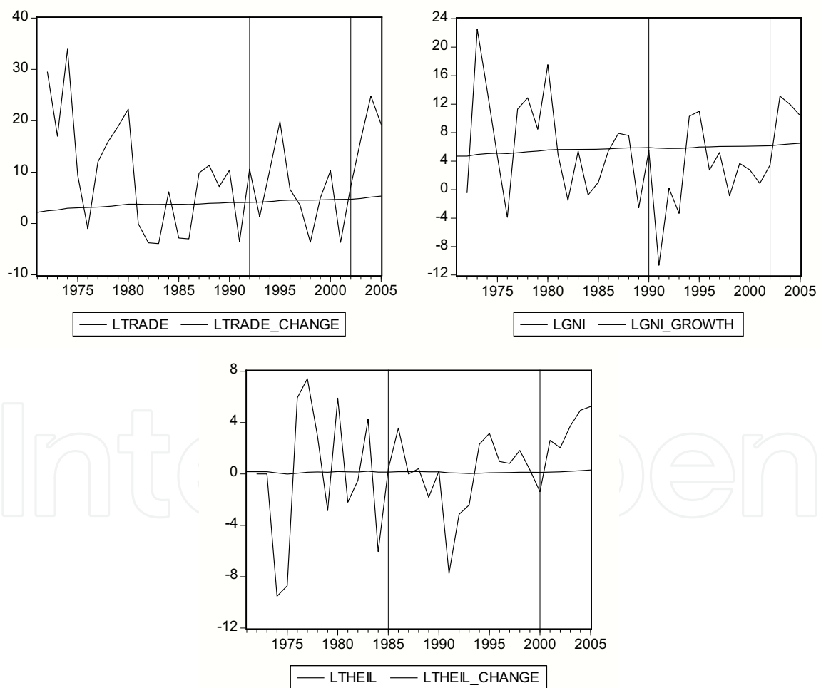
Fig. 3. Plots of the SAARC-5 Series and Endogenously Estimated Timing of Structural Breaks by the LP Test
