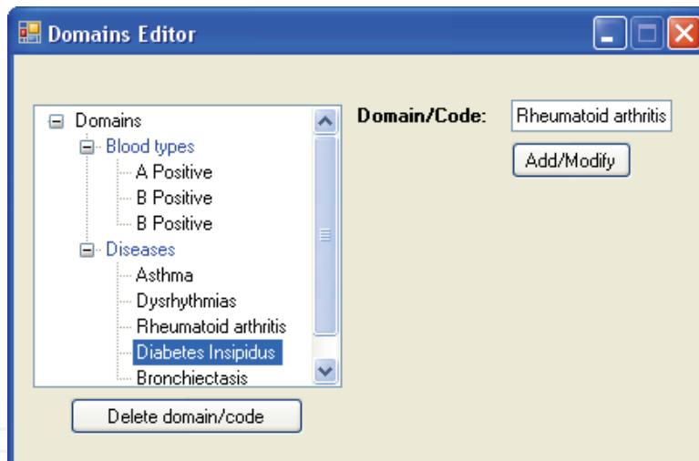
Fig. 3. Domains/codes editor
