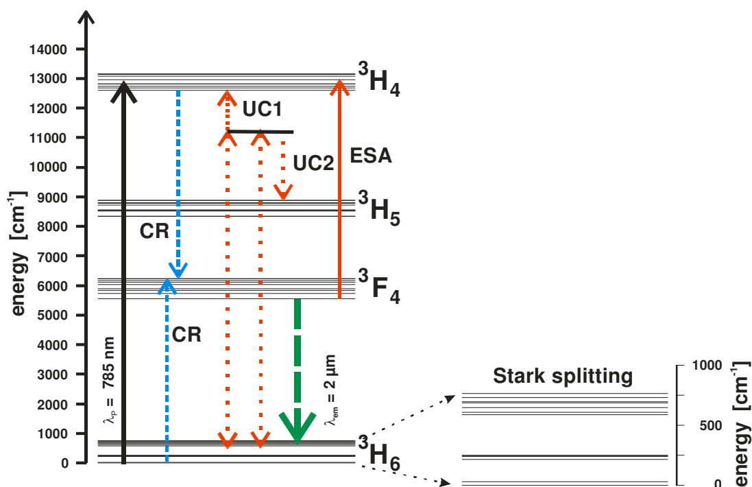
Fig. 2. Tm:YAG energy scheme with the relevant transitions for the 2\ \mu\text{m} laser emission and the Stark splitting of the ground state
