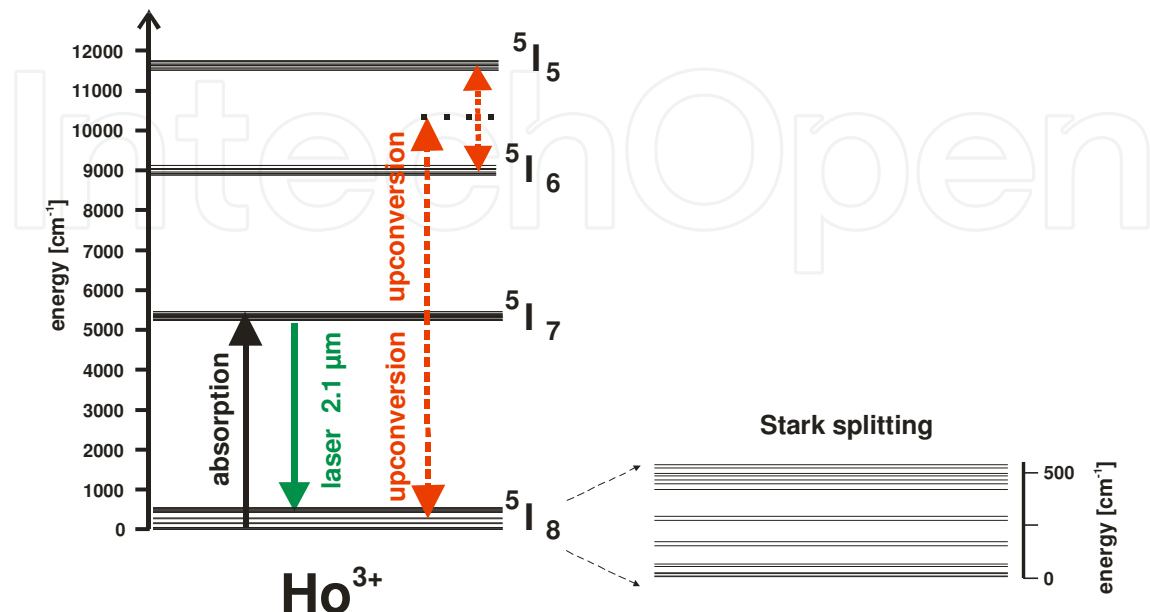
Fig. 6. Ho:YAG energy scheme with the relevant transitions for 2.1 \mu\text{m} laser operation
