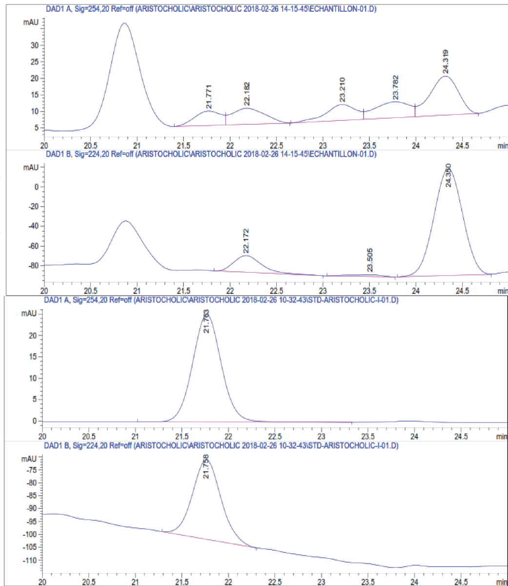
Figure 4. HPLC spectrum analysis of berztem roots and (AAI) standard. (Sigma A5512–25 mg Yellow powder lot # wxb6331V PCODE )
