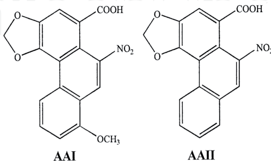
Figure 1. Chemical structure of nitrophenanthrene carboxylic acids.
