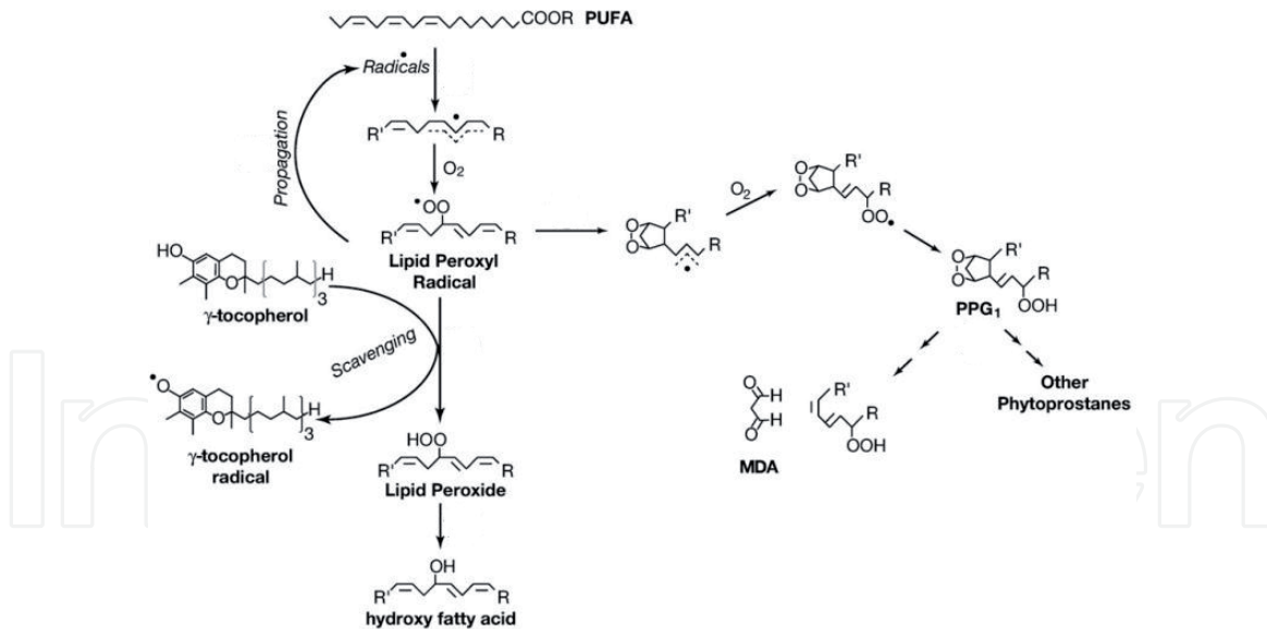
Figure 10. Lipid peroxidation [27].
