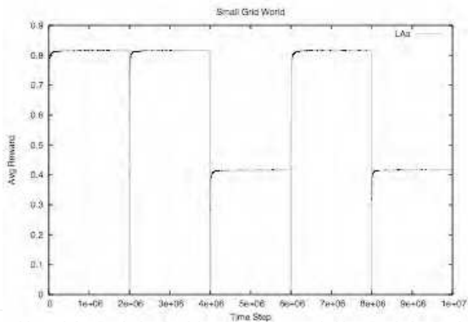
Fig. 4. Average Reward for the 2-location grid-world problem of Figure 3 .
