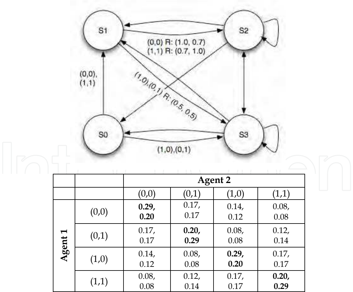
Fig. 1. A Markov Game Problem and its corresponding limiting game
