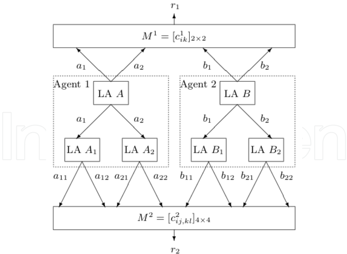
Fig. 5. An interaction between two agents constructed with a hierarchy of learning automata.
