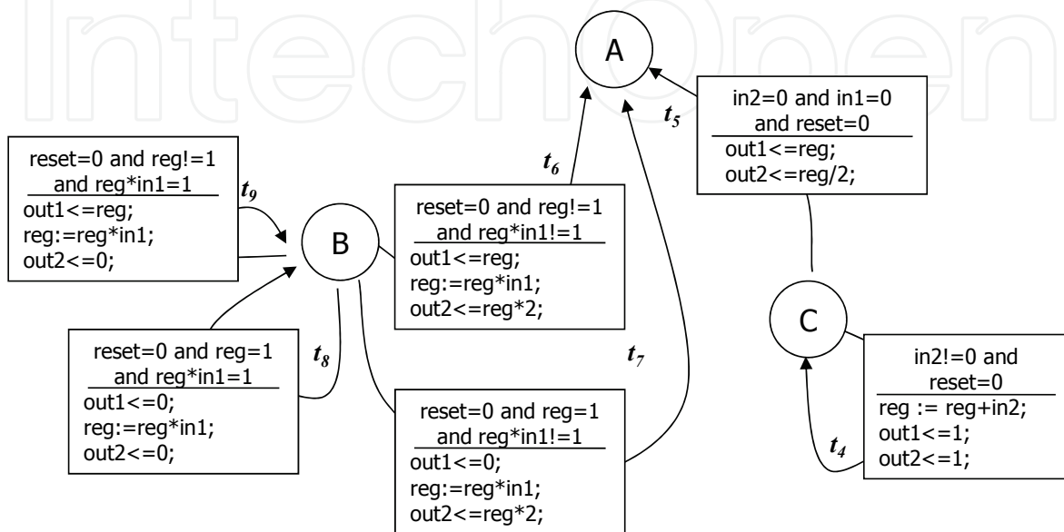
Fig. 18. Reduced EFSM.
