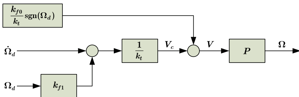
(a) open loop controller
