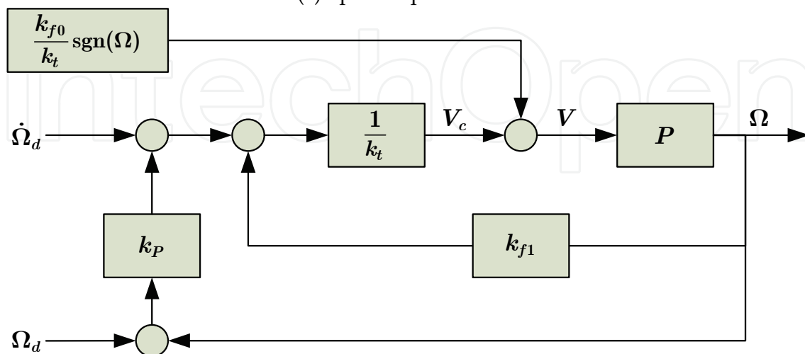
(b) closed loop controller
