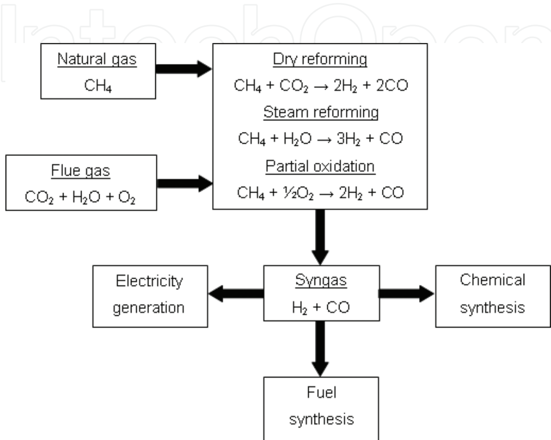
Figure 1. Tri-reforming of natural gas using flue gas from fossil fuel-based power plants.
