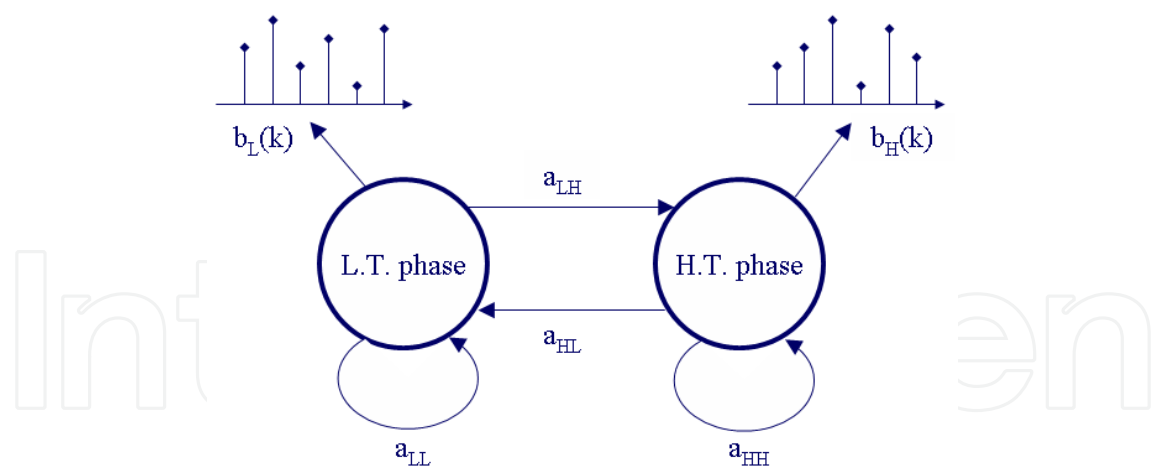
Fig. 11. A discrete hidden Markov model with two hidden phases for estimating biphasic property in a menstrual cycle from cutaneous temperature measurements.
