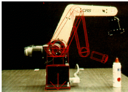
Figure 17. AR overlay in fixed environment for interactive path planning (Milgram, Zhai et al. 1993)
