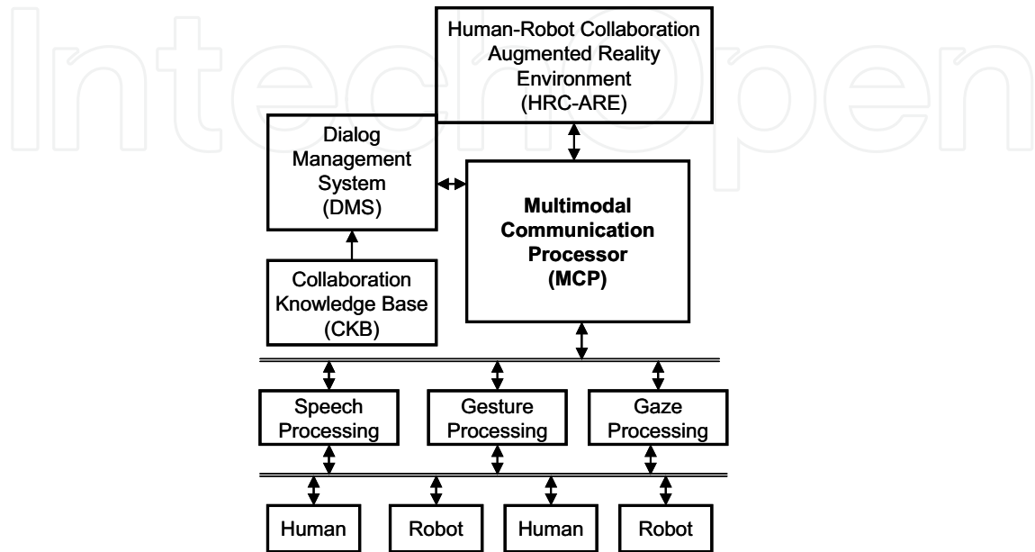
Figure 20. The Human-Robot Collaboration system architecture
