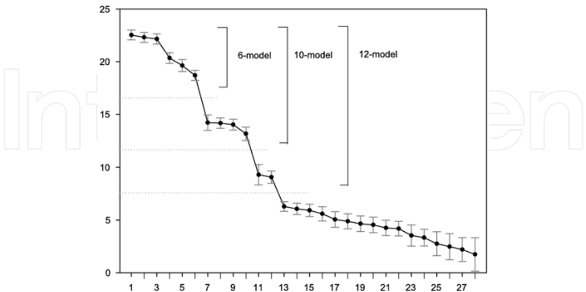
Fig. 3. Values for \bar{z} for each descriptor as a function of their order numbers. The relative deviations for \bar{z} in all the experiments are also displayed. The biggest gaps for \bar{z} and the models are outlined.
