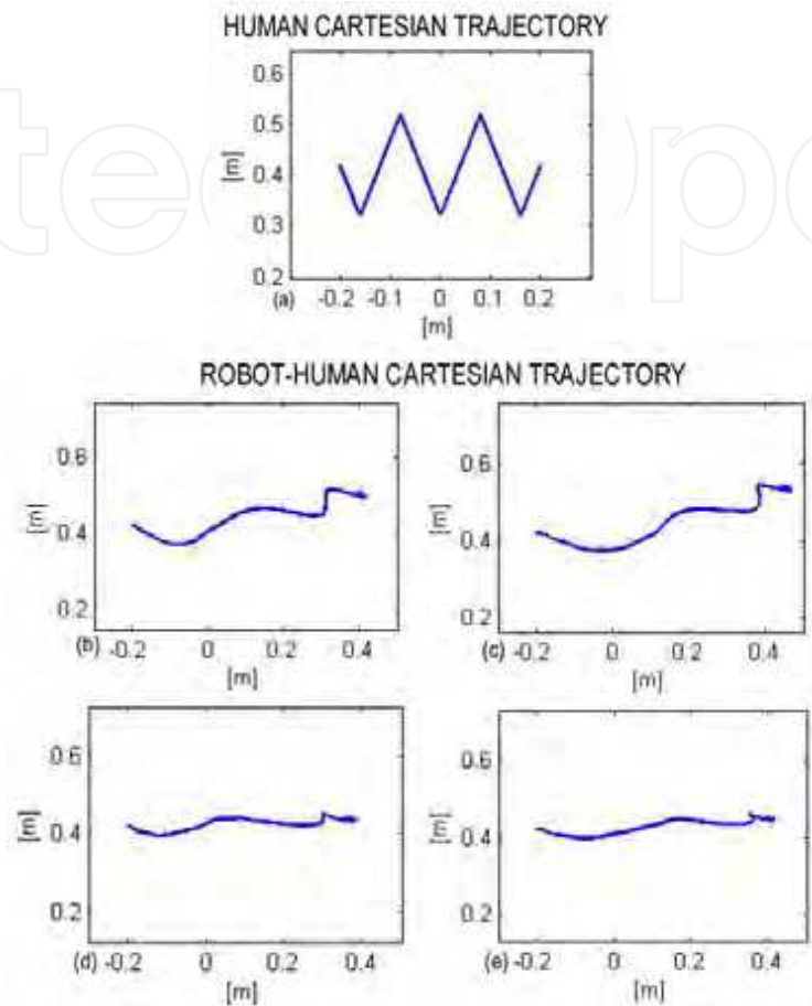
Fig. 16. Pathological trajectory (a) and subject trajectories counterbalanced by the robot for F_{dx} = 30 \text{ N} K_y = 100 \text{ N/m} (b), F_{dx} = 45 \text{ N} K_y = 100 \text{ N/m} (c), F_{dx} = 30 \text{ N} K_y = 1000 \text{ N/m} (d), F_{dx} = 45 \text{ N} K_y = 1000 \text{ N/m} (e) in case of severe disability.
