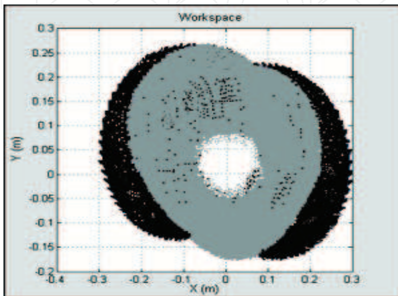
Fig. 5. MasterFinger-2 workspace. The black area represents the workspace covered by the up-elbow configuration and the grey area the one by the down-elbow configuration.
