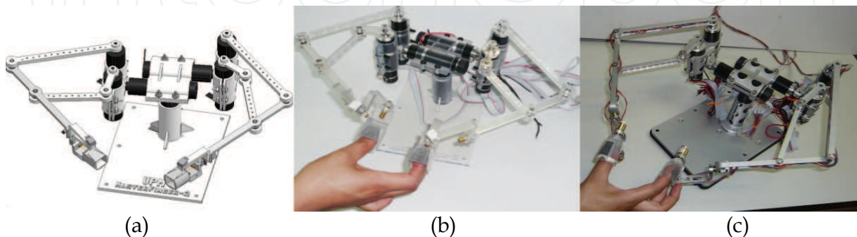
Fig. 4. Masterfinger-2: six degrees of freedom for each finger: (a). CAD model. (b). Resine prototype. (c).Aluminium prototype
