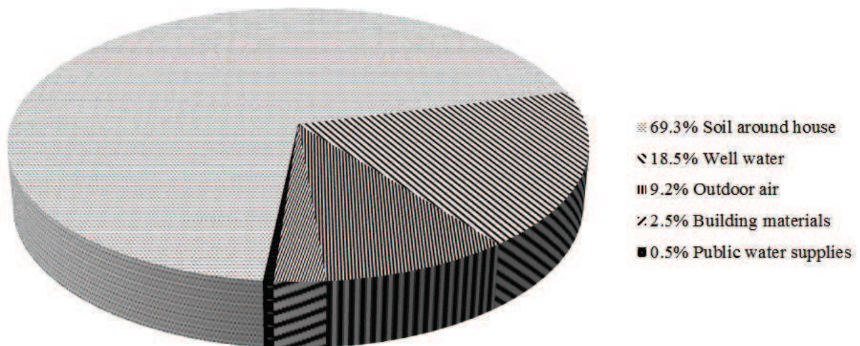
Figure 2. Radon source contribution in residential places.
