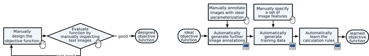
Figure 6. The traditional procedure for designing objective functions (left), and the proposed method for learning objective functions (right)
