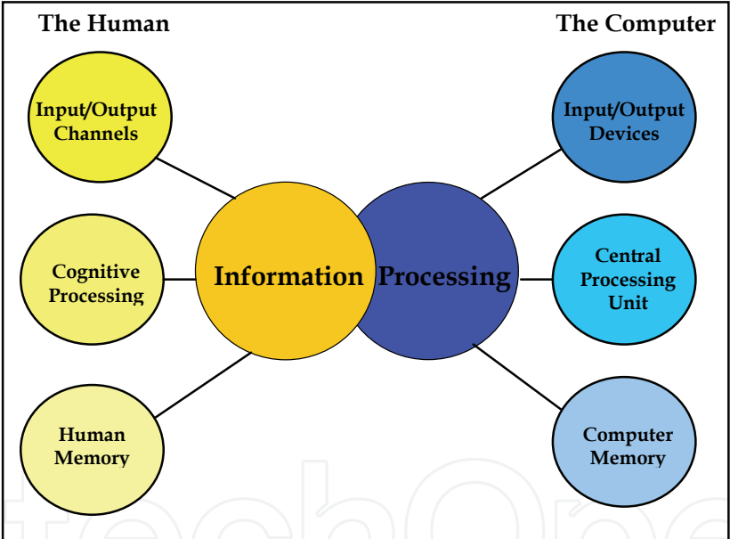
Figure 2. Information Processing
