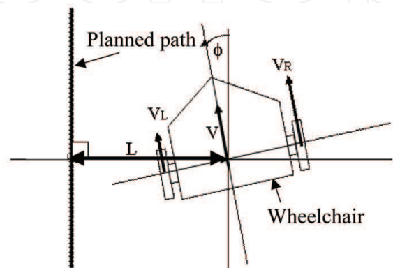
Fig.10. Trajectory following control method
