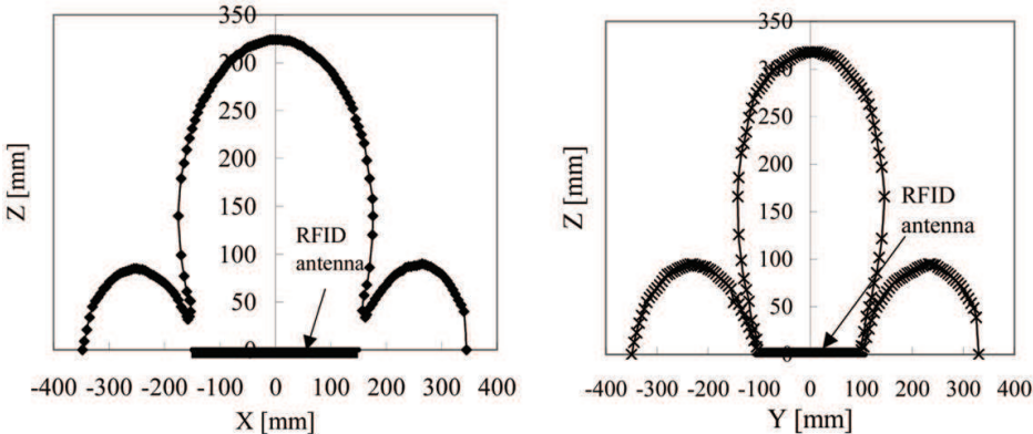
Fig. 7. Detection area of RFID antenna
