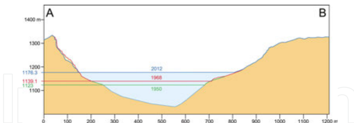
Figure 11. Profiles of Troitsky Crater in 1950, 1968, and 2012. The position of the A–B line is shown in Figure 10b.
