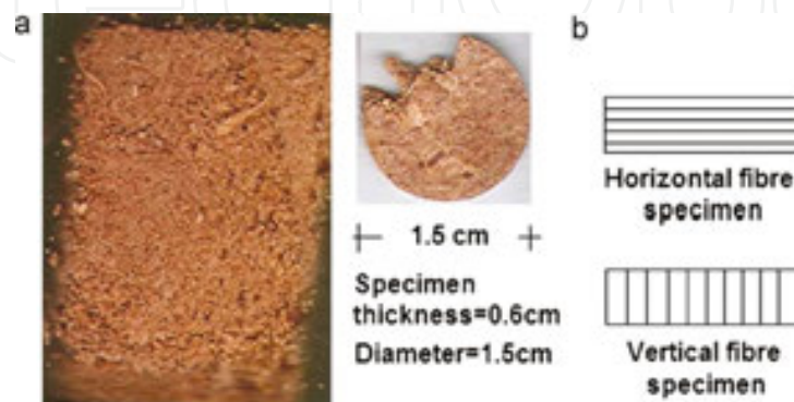
Figure 7. Material and specimen prepared for the study [37].
