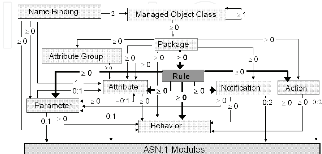
Fig. 6. Relations between proposed standard templates
