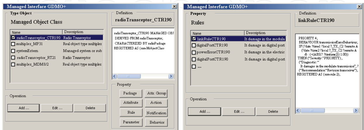
Fig. 13a System Object Classes Dialog Box
