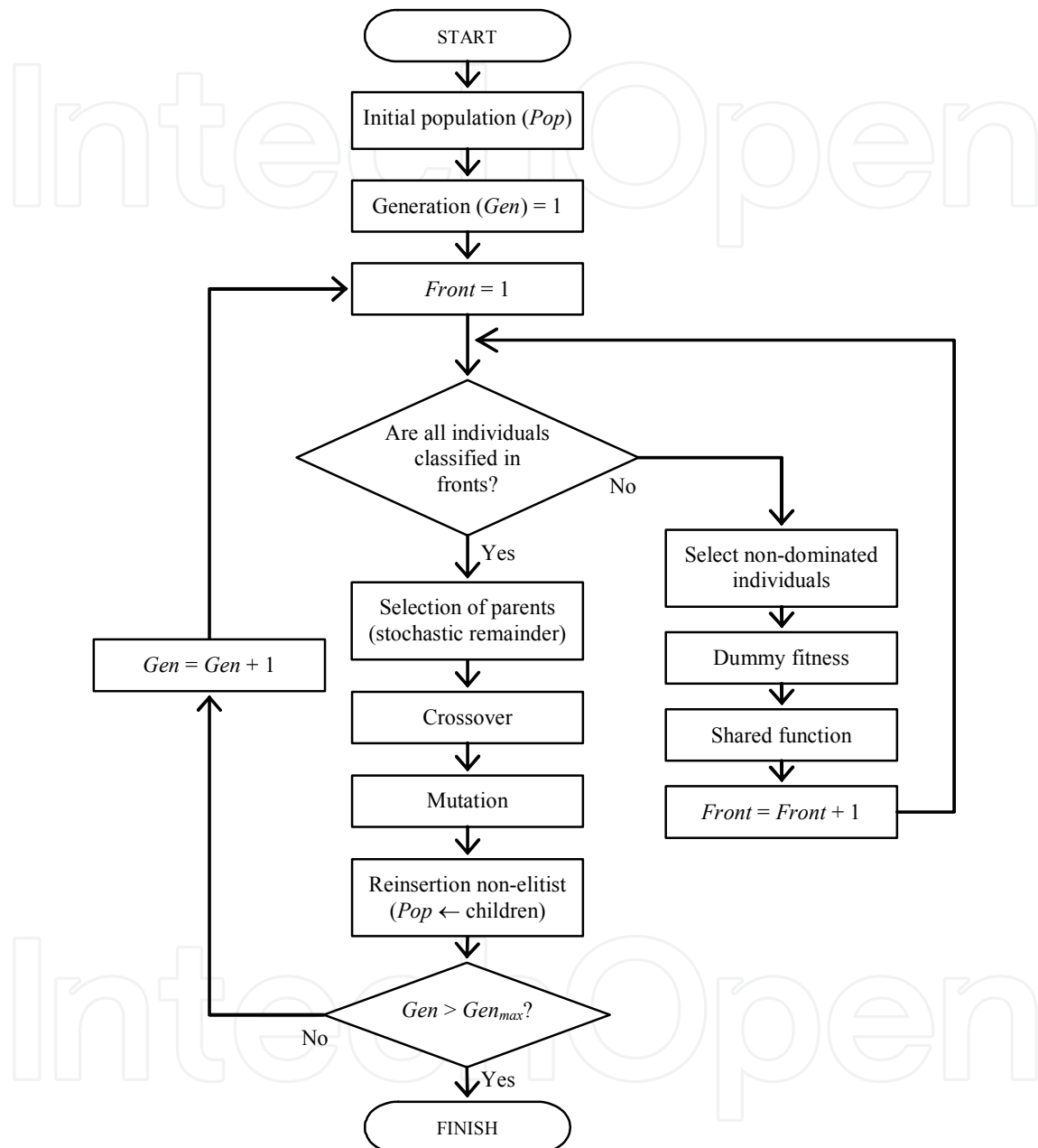
Fig. 2. NSGA's flow chart
