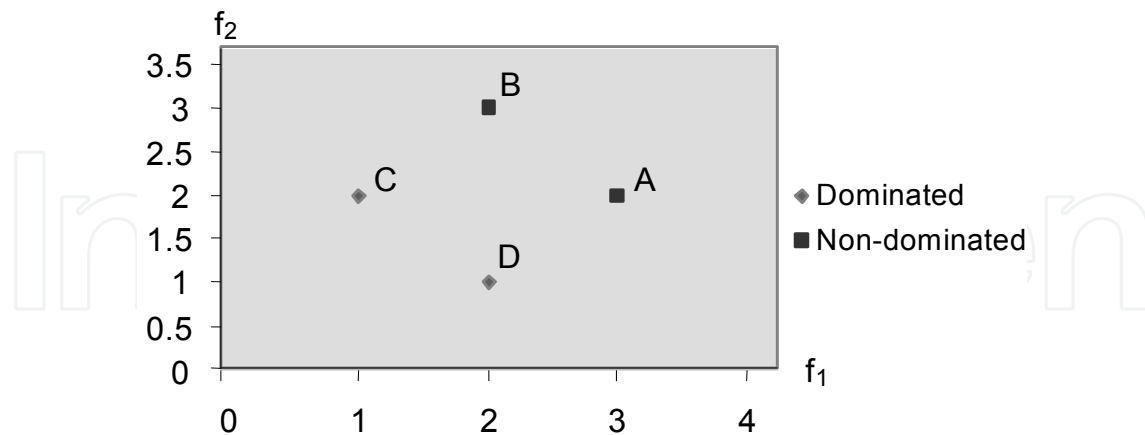
Fig. 1. Example of dominated and non-dominated solutions when maximizing f_1 and f_2 .
