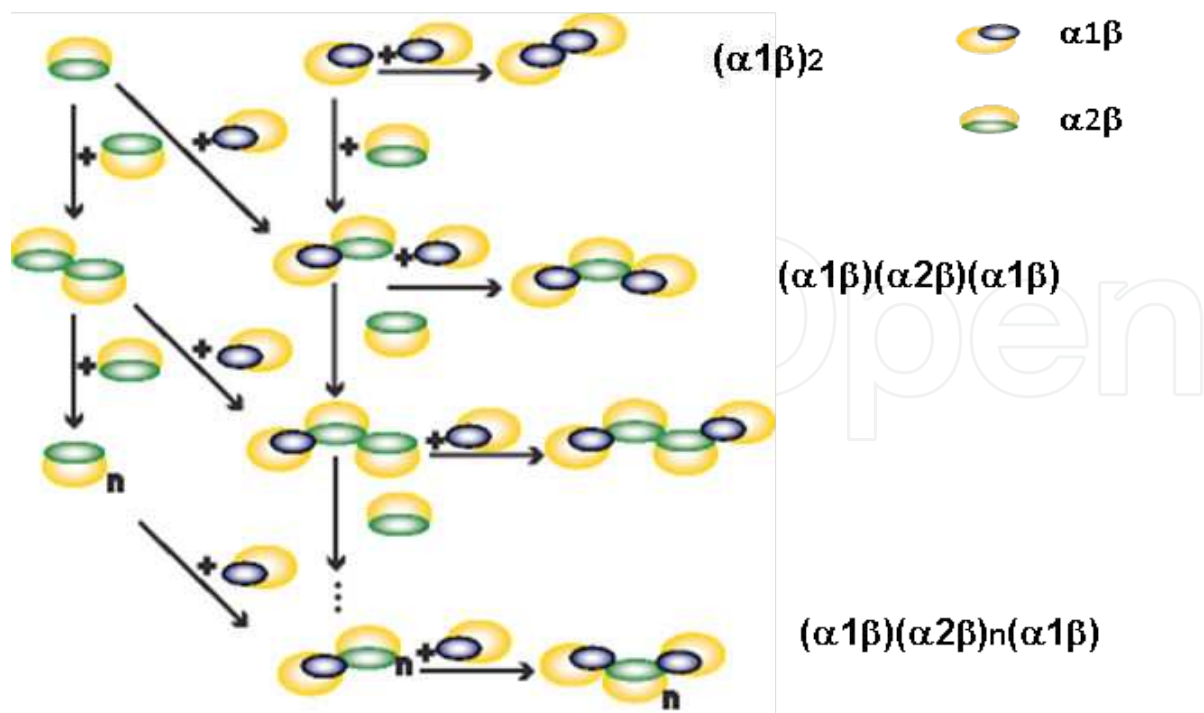
Figure 8. Proposed model for the formation of Hp 2-1 linear polymers. Nucleation occurs through the reaction between the two \alpha\beta units with the possible products: a simple (\alpha1\beta)2 dimer is initially formed without further extension because of the saturation of free -thiol groups. The next linear trimer is formed with the addition of two (\alpha1\beta) units to one (\alpha2\beta) . Notably, either (\alpha1\beta) or (\alpha2\beta) may subsequently add to one (\alpha2\beta) unit until both ends are bound with (\alpha1\beta) .
