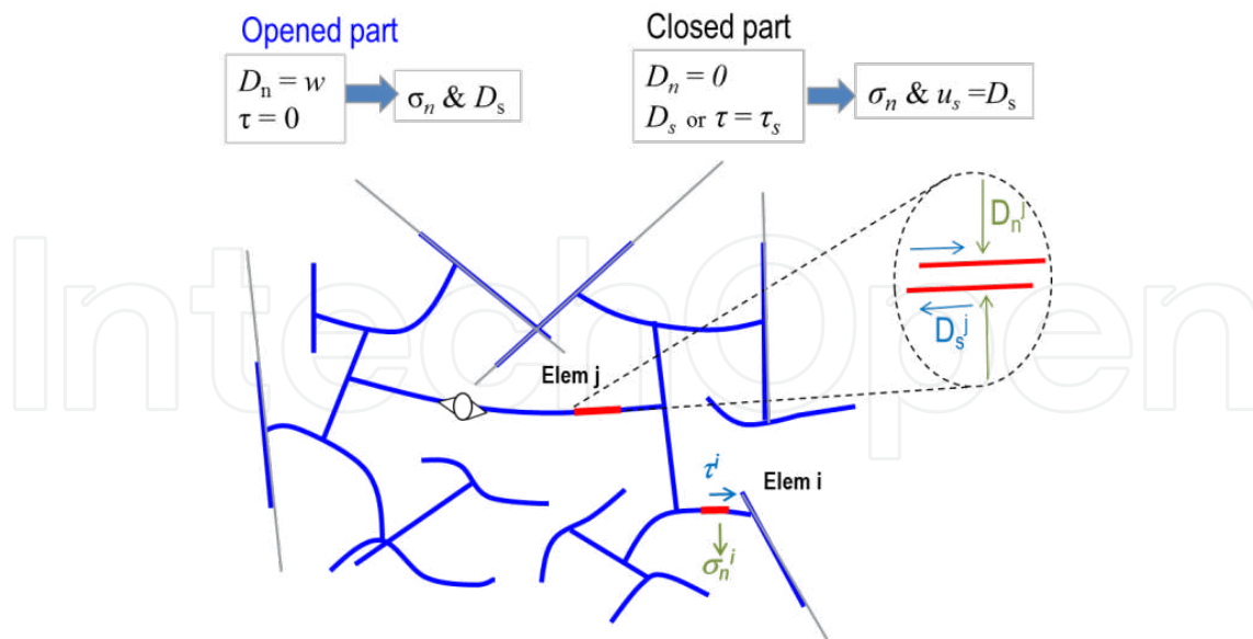
Figure 3. Stress Shadow Effect from opened (blue) HFN and closed parts (grey) of intercepted NFs
