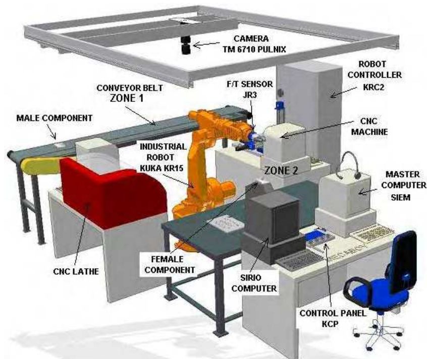
Figure 1. Manufacturing cell
