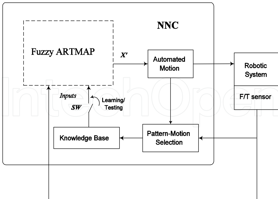
Figure 8. System Structure
