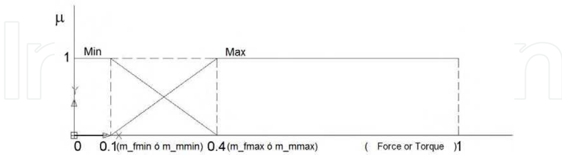
Figure 6. Membership functions
