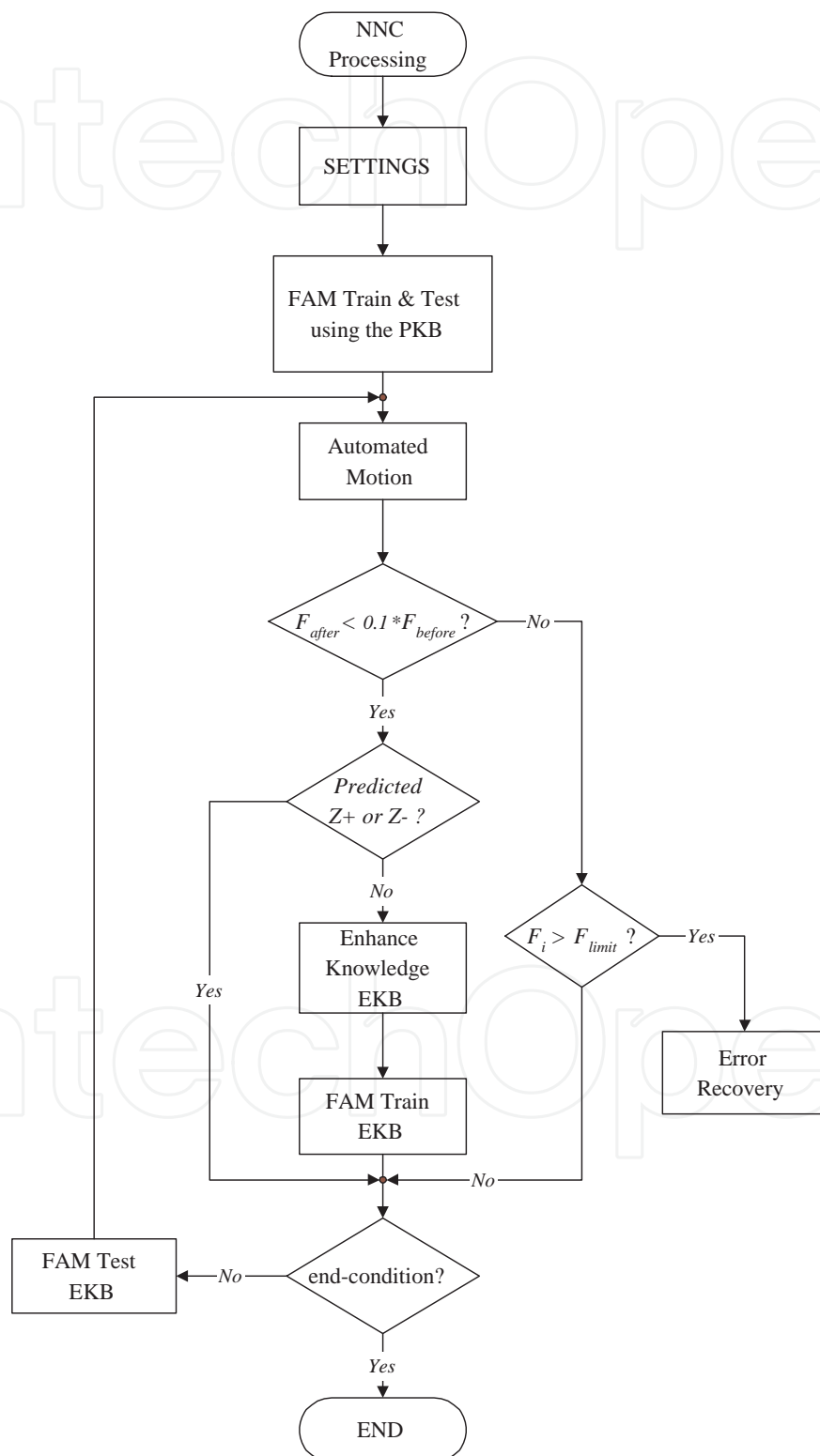
Figure 9. Flowchart of the NNC processing
