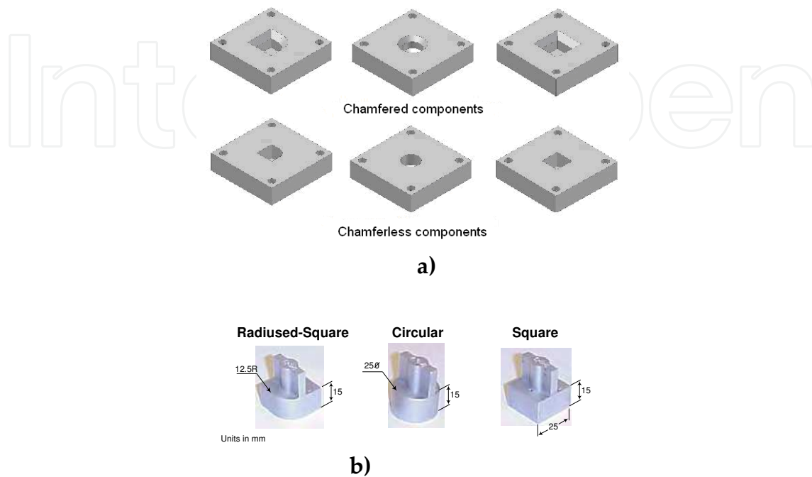
Figure 2. a) Female assembly components, b) Male assembly components
