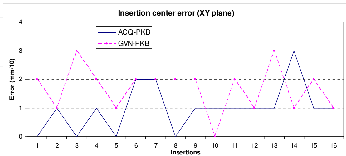
Figure 15. Insertion center error on XY plane
