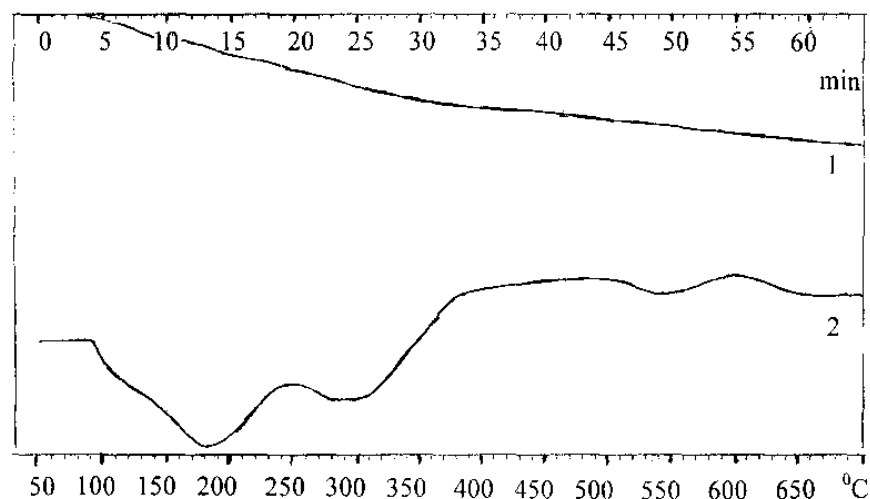
Figure 1. Derivatogram of natural zeolite. 1 – TG; 2 – DTA.
