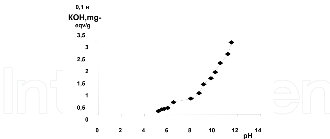
Figure 4. Potentiometric titration curve of the H + form of zeolite.
