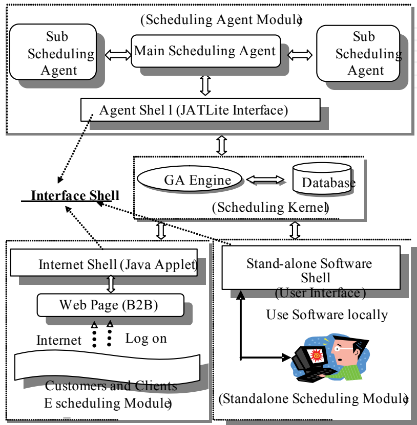
Figure 5. Scheduling agent
