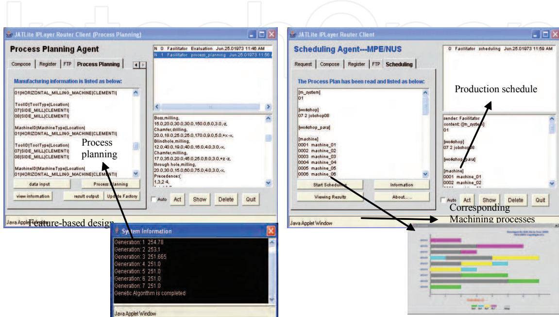
Figure 7. Optimal process plans and production schedules generated from the PPA and MSA respectively
