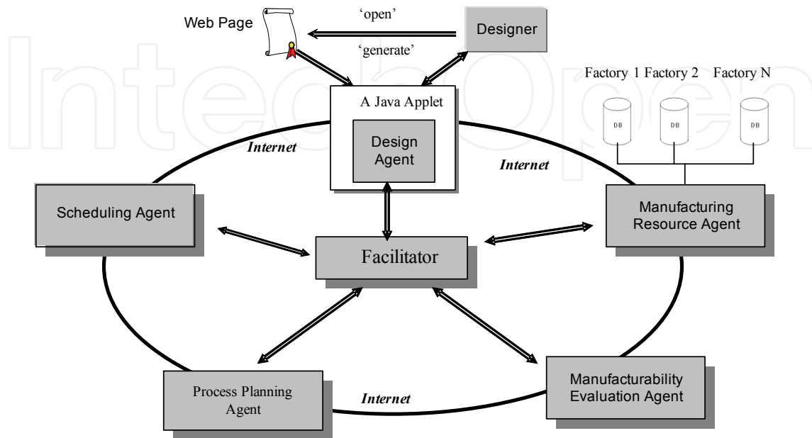
Figure 3. System architecture
