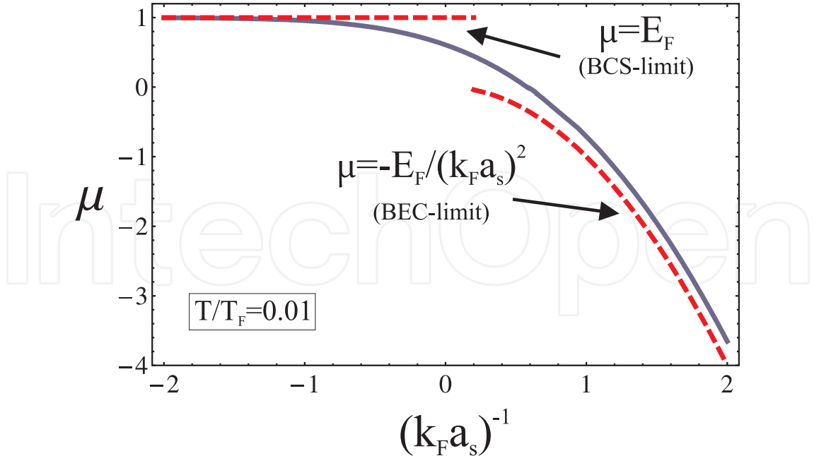
Figure 5. The chemical potential \mu is shown as a function of the interaction parameter 1/(k_F a_s) , for a low temperature and a balanced gas ( \zeta = 0 ). In the regime of negative a_s the chemical potential tends to the Fermi energy, as in the BCS theory. For positive a_s , the chemical potential tends to the binding energy of the strongly bound ‘Cooper molecules’ that Bose-Einstein condense to form a superfluid.
