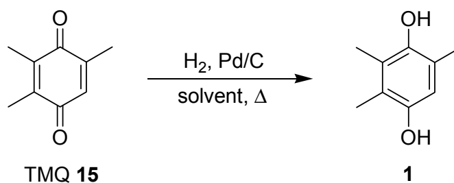
Scheme 3. Catalytic hydrogenation of TMQ to TMHQ.
