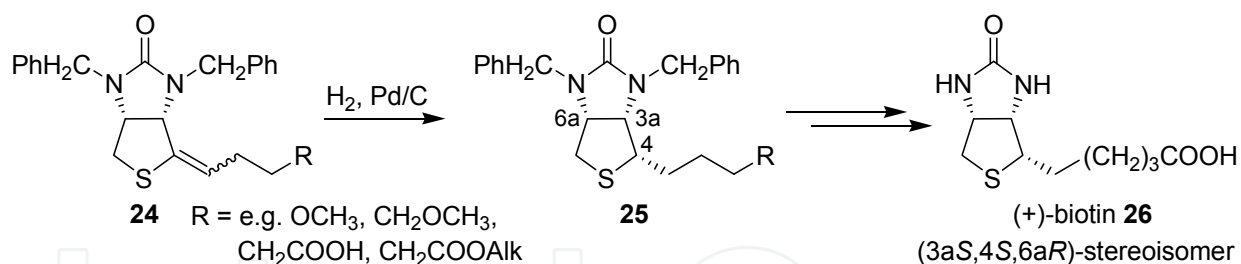
Scheme 6. Stereoselective heterogeneous hydrogenation in routes towards (+)-biotin.
