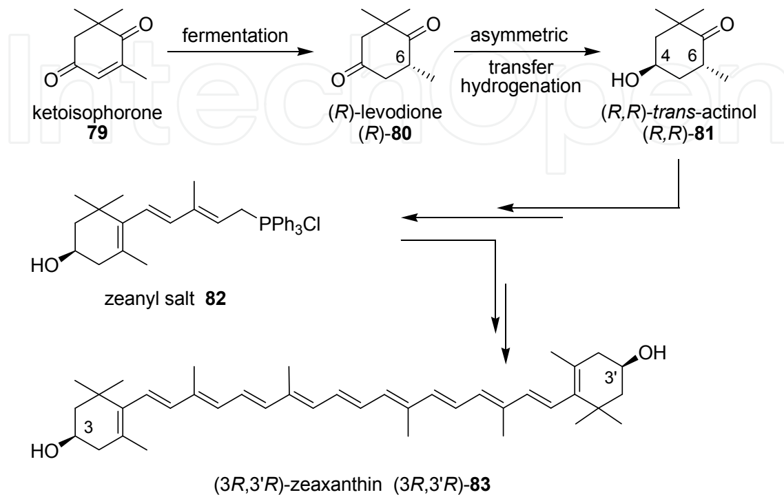
Scheme 23. Asymmetric transfer hydrogenation of ( R )-levodione in the synthesis of ( 3R,3'R )-zeaxanthin.
