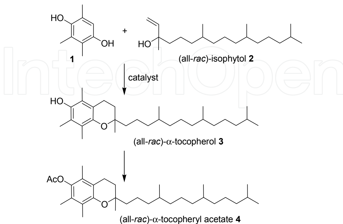
Scheme 1. Final steps of the chemical production of vitamin E.
