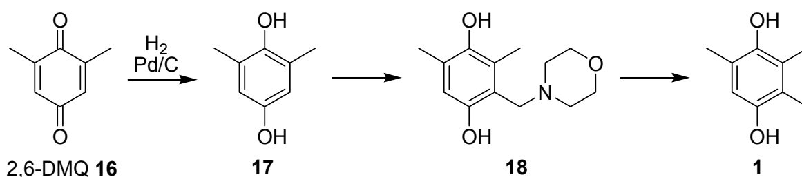
Scheme 4. Synthesis of TMHQ from 2,6-DMQ.
