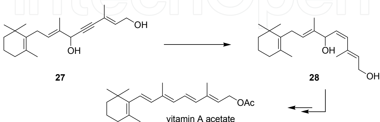
Scheme 7. Semi-hydrogenation of a vitamin A intermediate.
