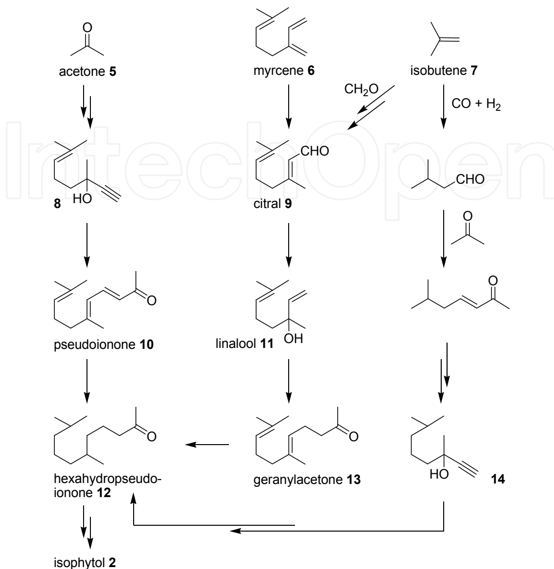
Scheme 2. Synthesis of isophytol ( E/Z isomerism of olefins is omitted here).
