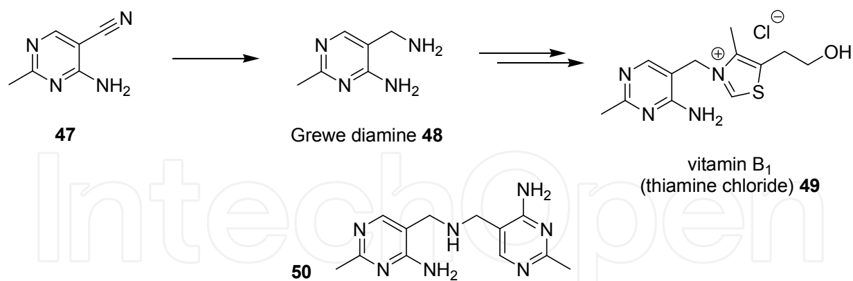
Scheme 15. Production of Grewe diamine for vitamin B 1 .
