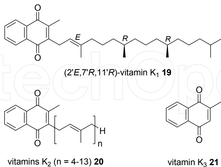
Figure 1. Molecular structures of the different K vitamins.
