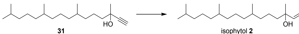
Scheme 9. Preparation of isophytol by semi-hydrogenation.
