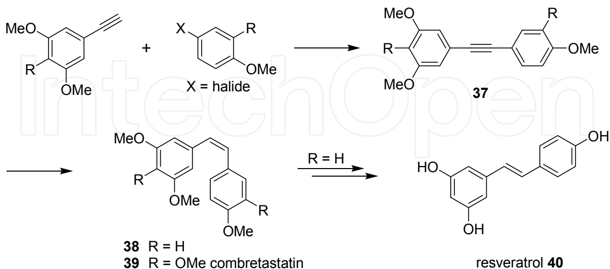
Scheme 12. Synthesis of combretastatin and resveratrol via Sonogashira coupling and semi-hydrogenation.
