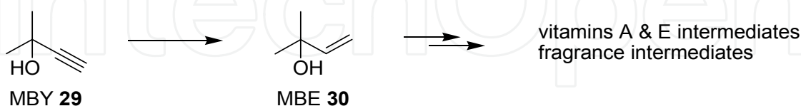
Scheme 8. Semi-hydrogenation of MBY.
