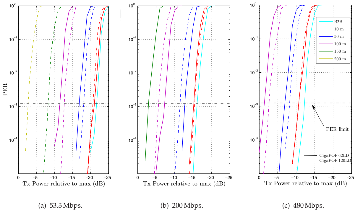
Figure 7. PER vs. transmitted power after a 1 meter wireless link for transmission rates of 53.3, 200 and 480 Mbps for both GigaPOF-62LD and GigaPOF-120LD.
