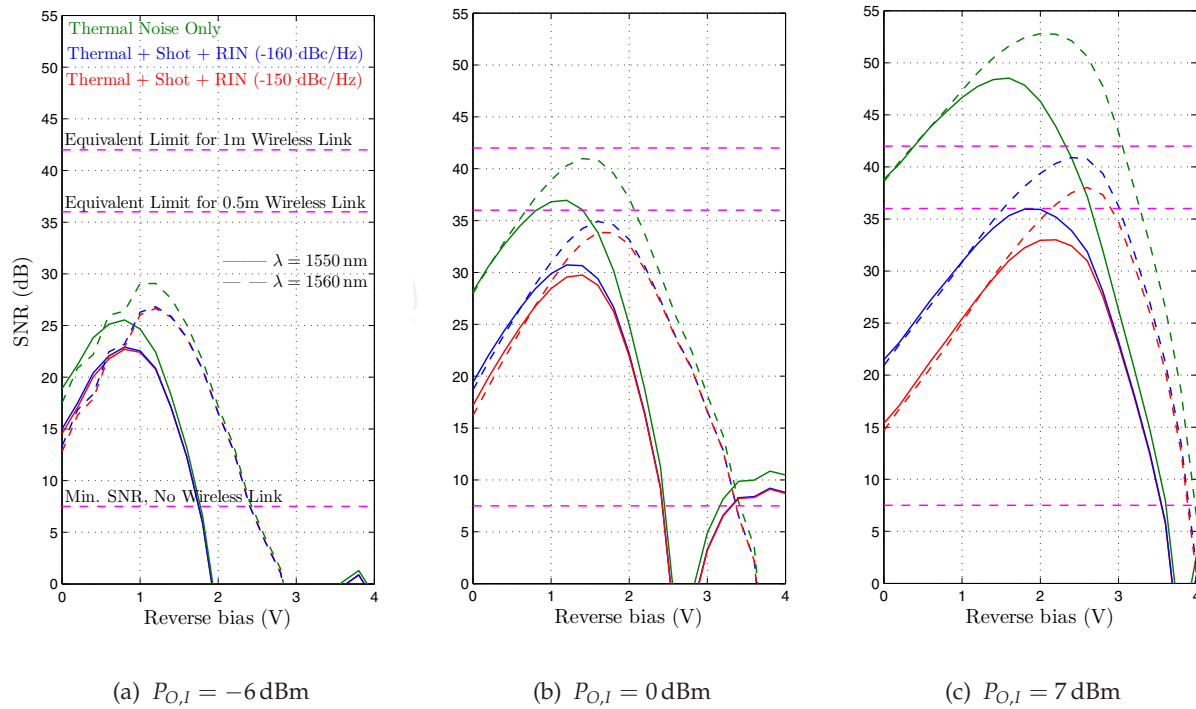
Figure 18. SNR as a function of reverse bias for three different values of optical input power.
