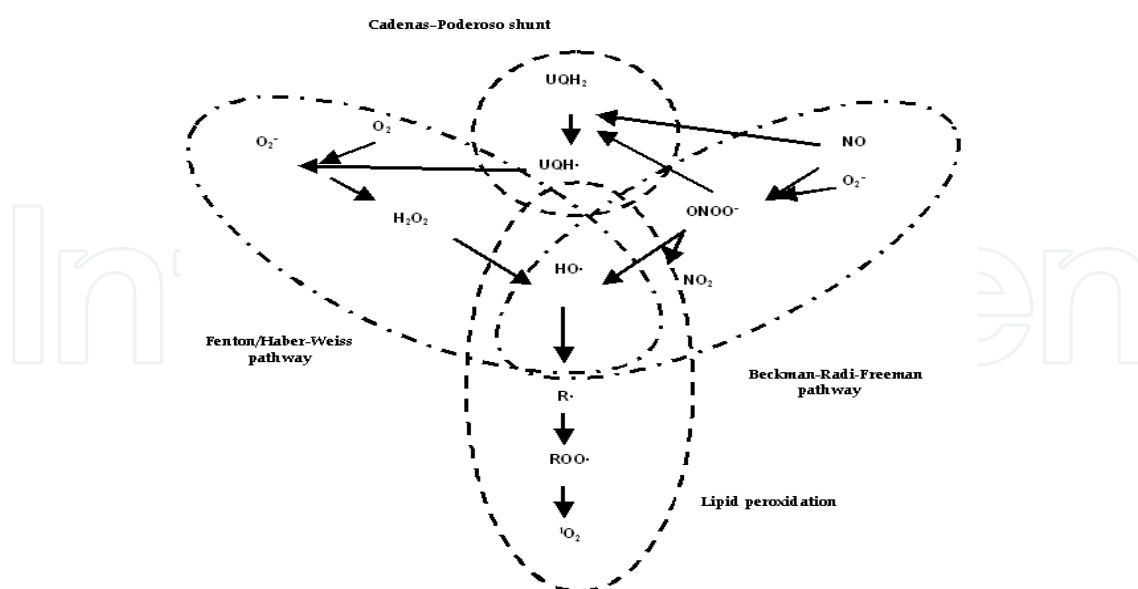
Figure 3. The free-radical mediated chain reaction in biochemistry. O_2^- , superoxide radical; H_2O_2 , hydrogen peroxide; HO\cdot , hydroxyl radical; NO, nitric oxide; ONOO^- , peroxynitrite; \cdot NO_2 , nitrogen dioxide; UQH 2 , ubiquinol; UQH \cdot , ubisemiquinone; R \cdot , alkyl radical; ROO\cdot , peroxy radical; ^1O_2 , singlet oxygen.
