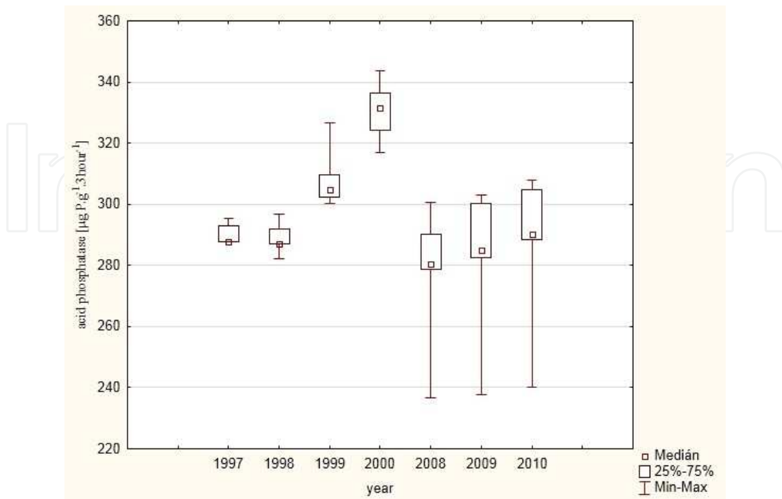
Figure 11. Acid phosphatase activity of soil in the monitored area situated in a marginal region of north-eastern Slovakia expressed by descriptive statistics
