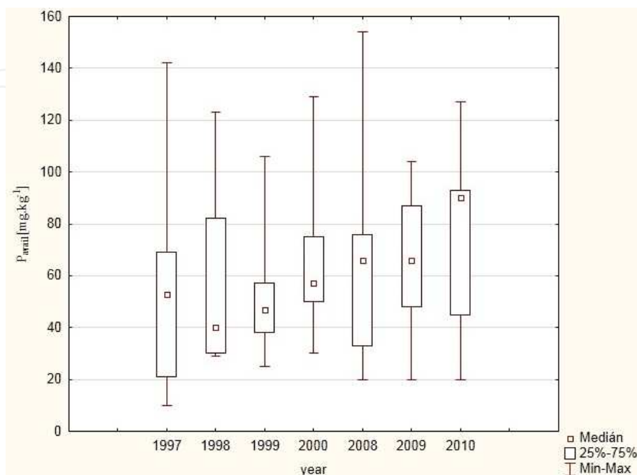
Figure 6. P_{\text{avail}} content of soil in the monitored area situated in a marginal region of north-eastern Slovakia expressed by descriptive statistics
