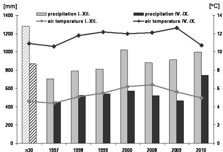
Figure 1. The course of average air temperatures (°C) and sum of precipitation (mm) during the observed period in the observed area situated in a marginal region of north-eastern Slovakia
