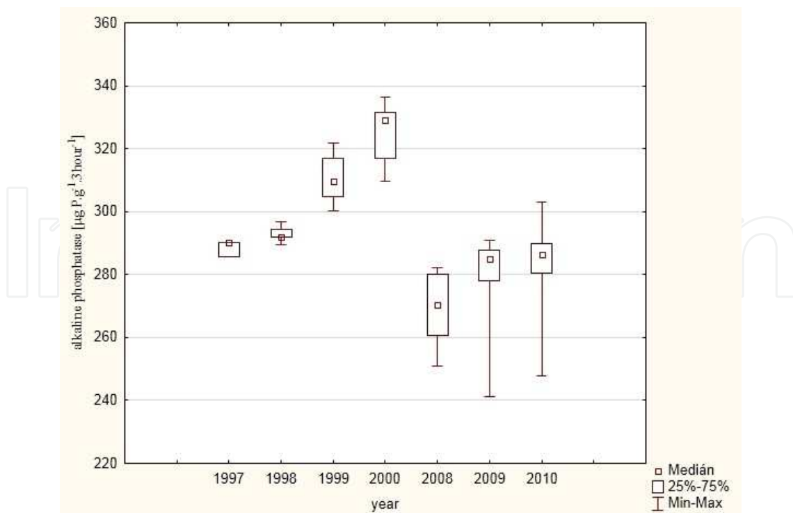
Figure 12. Alkaline phosphatase activity of soil in the monitored area situated in a marginal region of north-eastern Slovakia expressed by descriptive statistics
