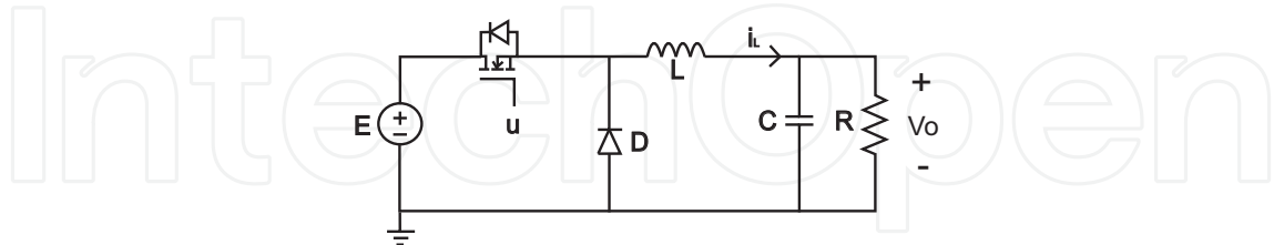
Fig. 1. The electrical circuit of the “buck” converter.
