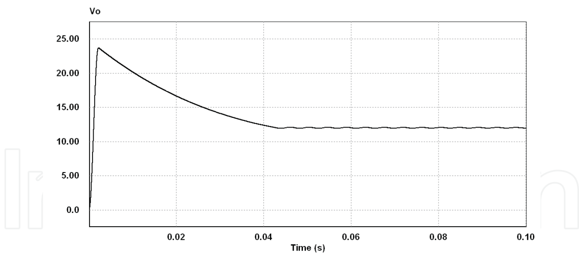
Fig. 7. Output voltage of buck converter in open-loop.
