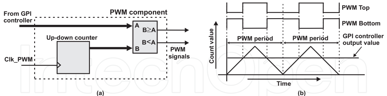
Fig. 17. (a) PWM component; (b) PWM outputs.
