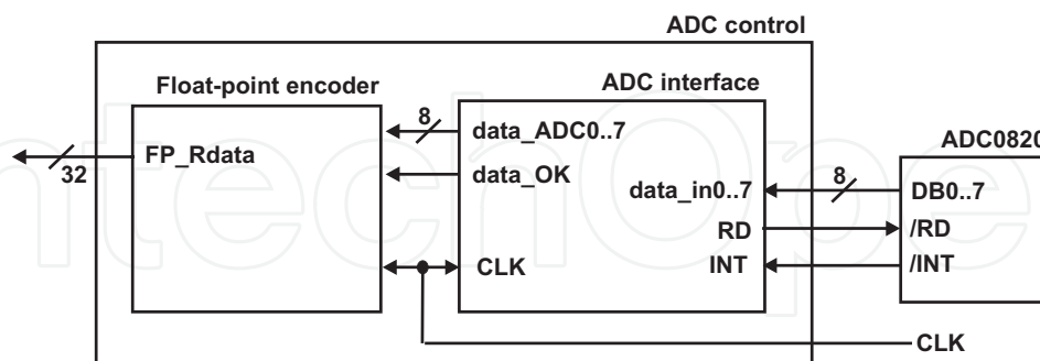
Fig. 12. Block Diagram of the ADC control component.
