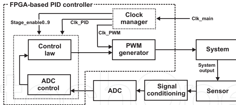
Fig. 11. Block diagram of FPGA-based PID controller.
