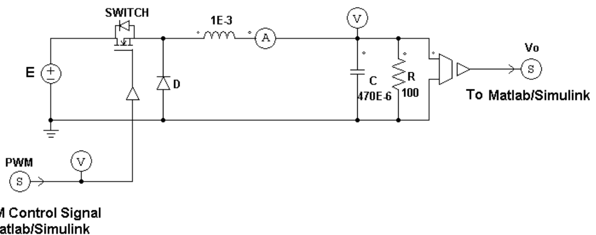
Fig. 4. Buck converter circuit for cosimulation with Simulink.
