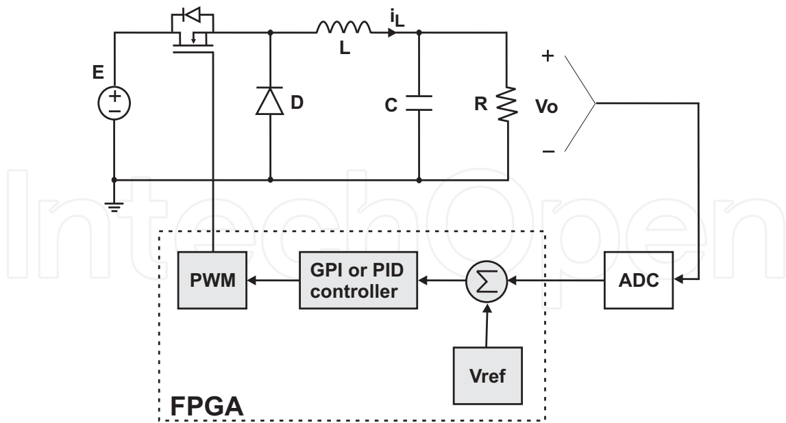
Fig. 18. Block diagram of the FPGA-based control system for PID controller.
