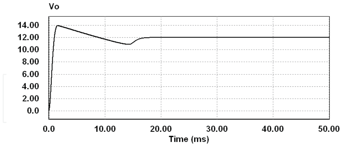
Fig. 8. Output voltage of buck converter with PID controller in cosimulation.
