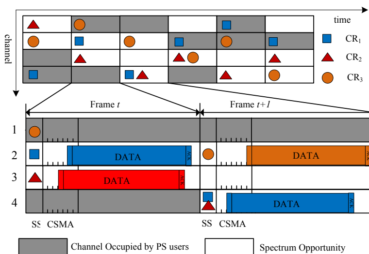
Fig. 6. Cognitive CSMA-based McMAC protocol for CRN
