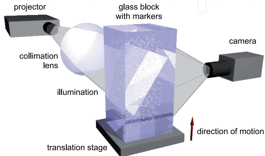
Fig. 9. Sketch of the experimental setup: A video projector is imaging different illumination profiles into the measurement volume, which is observed by a digital camera. A glass block with internal markers is translated vertically through the measurement volume.
