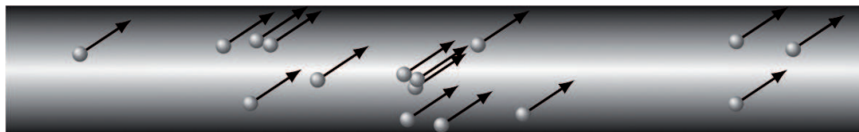
(a) Particles having an out-of-plane velocity component
