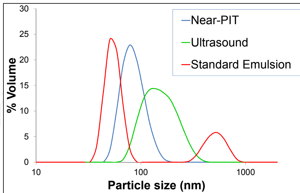
Fig. 10. Influence of emulsification process in particle size distribution, nanoemulsion formulation: \phi_{\text{oil}} = 0.35 , X_{\text{Brij 700}} = 0.4 and 5.2 wt% surfactant concentration. (Adapted from Galindo-Alvarez, et al., 2011)
