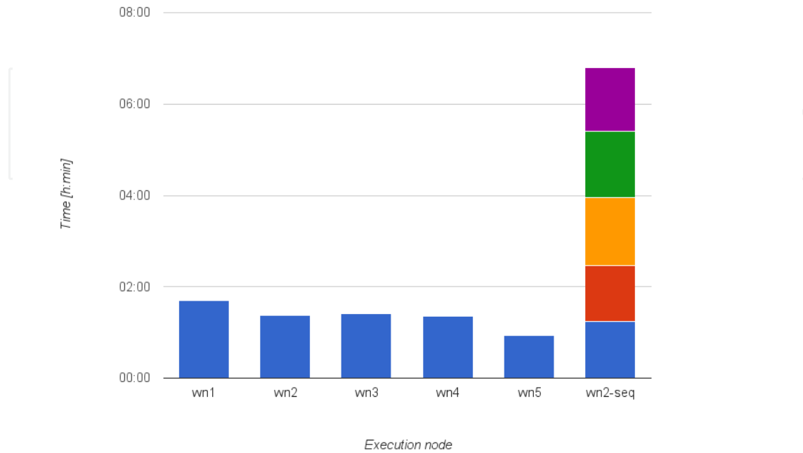
Fig. 7. Total execution time comparison between grid environment and sequential execution
