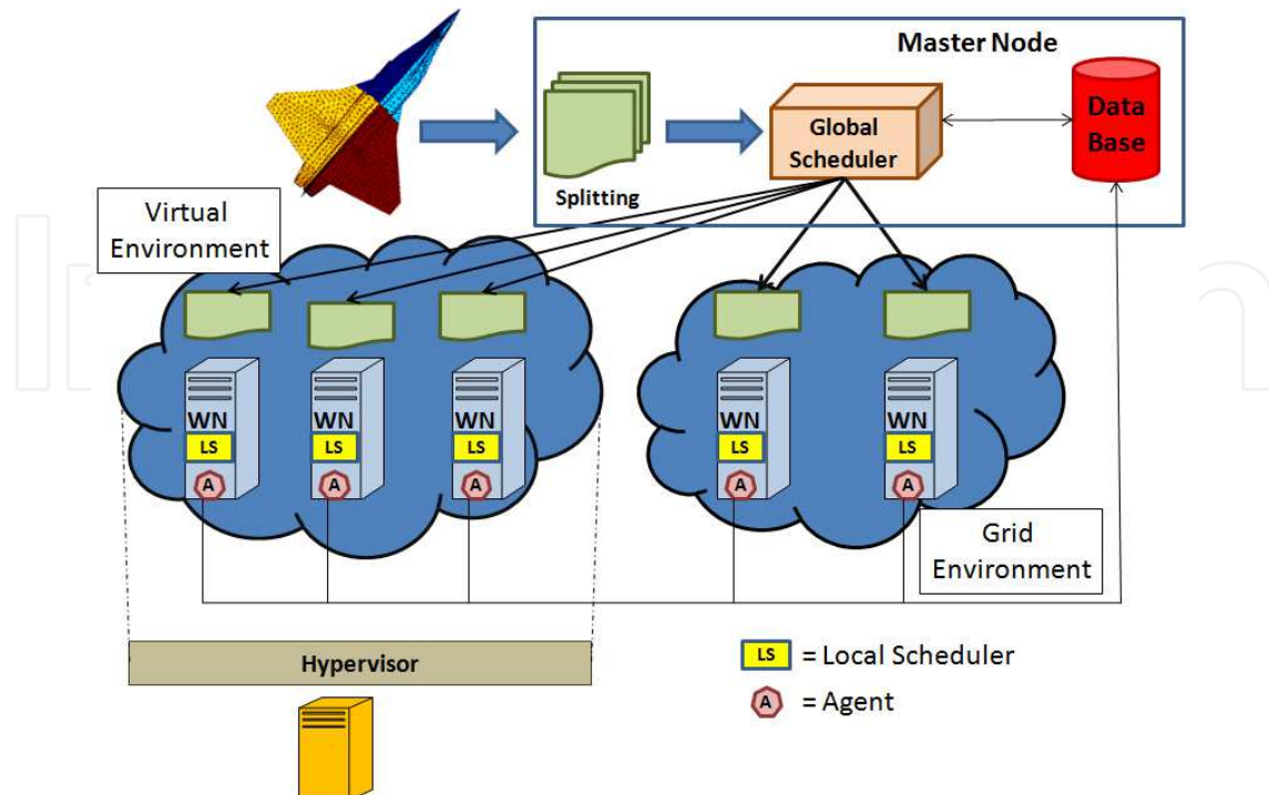
Fig. 6. GridCEM Architecture.
