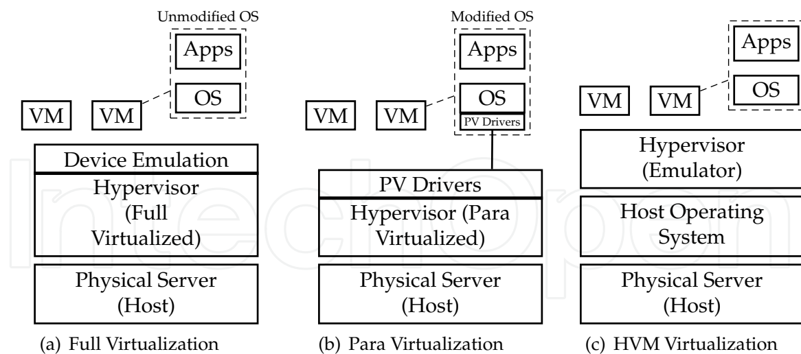
Fig. 3. Virtualization approaches.
