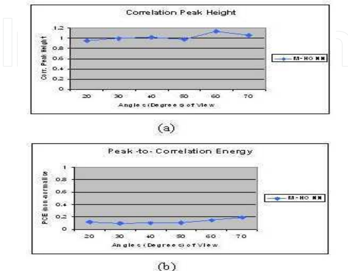
Fig. 7. (Adapted by Kypraios et al., 2008) shows (a) correlation peak-height versus the out-of-plane rotation angles of the object over the range of 20^\circ to 70^\circ . We tested the M-HONN system with the true-class object's intermediate car poses over the same range out-of-plane rotated at 10^\circ increments; (b) the non-normalised PCE values of the test images at 10^\circ increments versus the angles of view over the range of 20^\circ to 70^\circ .
