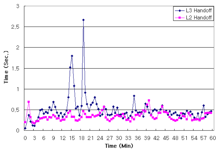
Fig. 7. Packet delay on conversational traffic class
