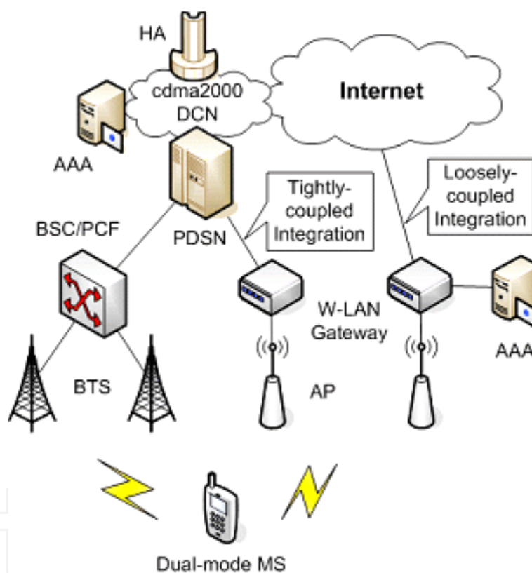
Fig. 1. Interworking architecture of heterogeneous wireless networks
