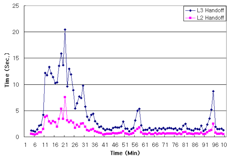
Fig. 9. Packet delay on interactive traffic class
