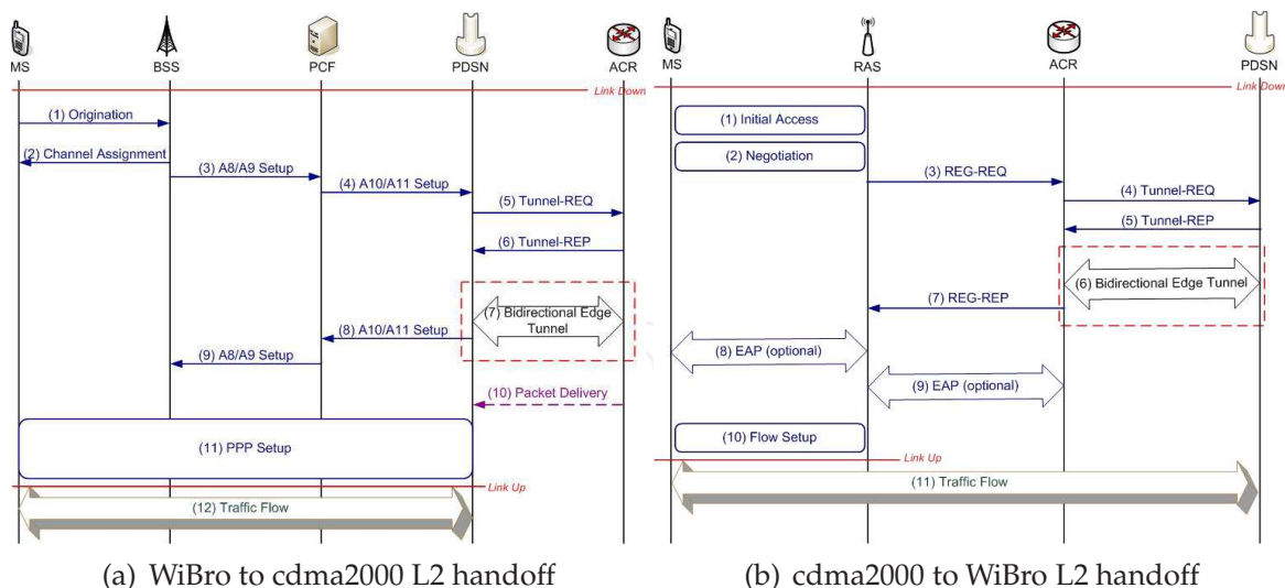
Fig. 4. L2 handoff procedure
