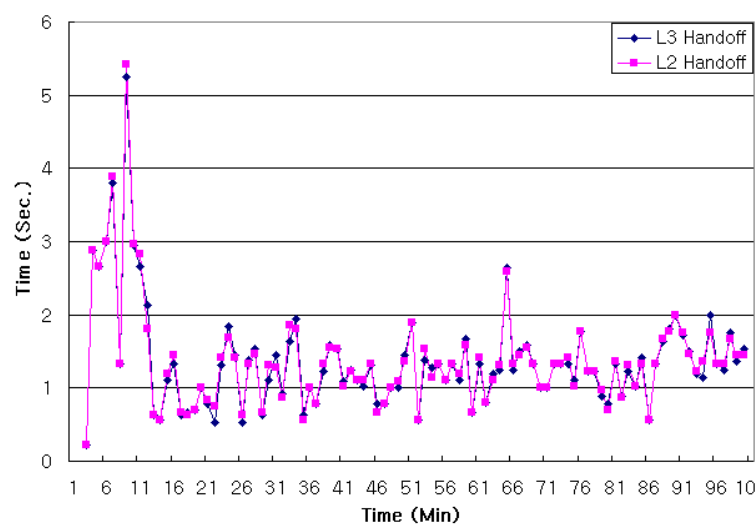
Fig. 10. Packet delay on background traffic class
