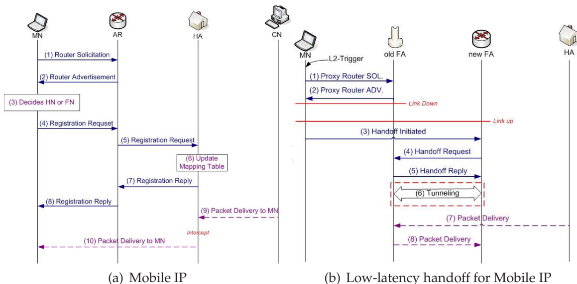
Fig. 2. L3 handoff procedure
