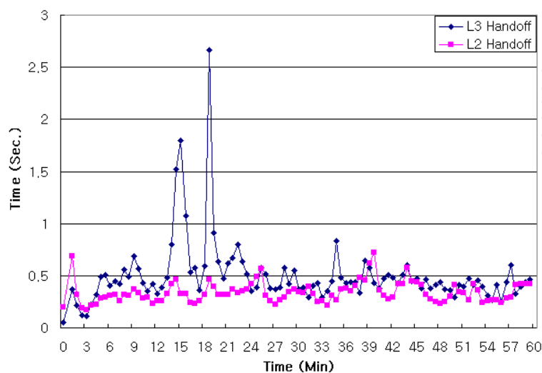
Fig. 8. Packet delay on streaming traffic class
