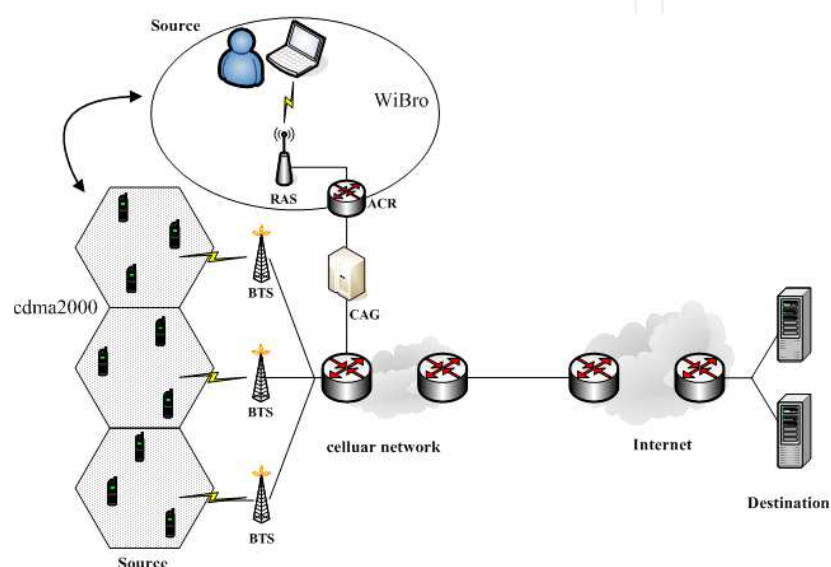
Fig. 5. Simulation model for performance evaluation
