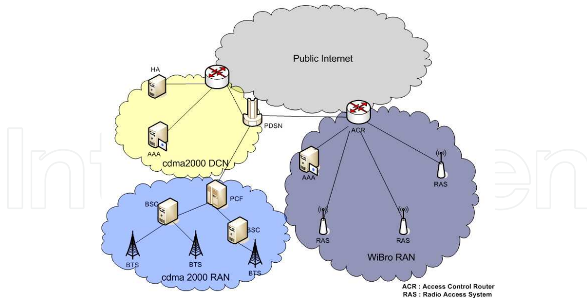
Fig. 3. Interworking Architecture between cdma2000 and WiBro networks
