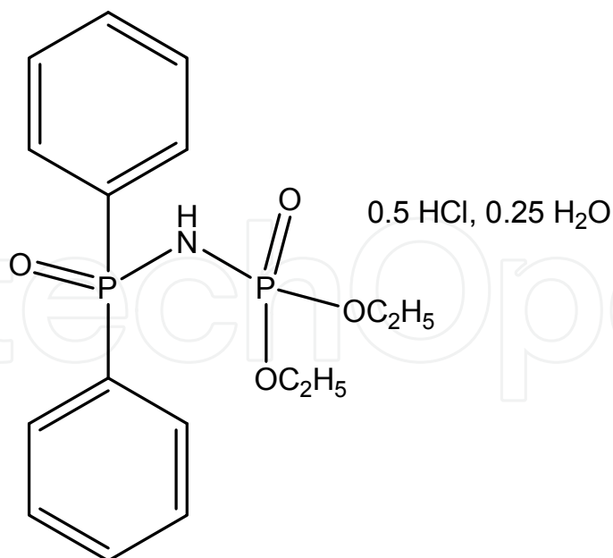
Scheme 35. Refcode WIYFAL [128]
