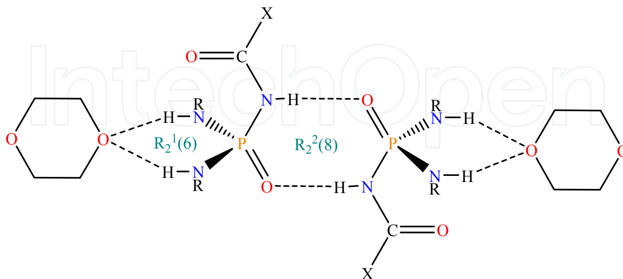
Scheme 13. A four-component cluster in the solvated molecule CCl_3C(O)NHP(O)[NHC_6H_{11}]_2 \cdot C_4H_8O_2 ( X = CCl_3 , R = C_6H_{11} )
