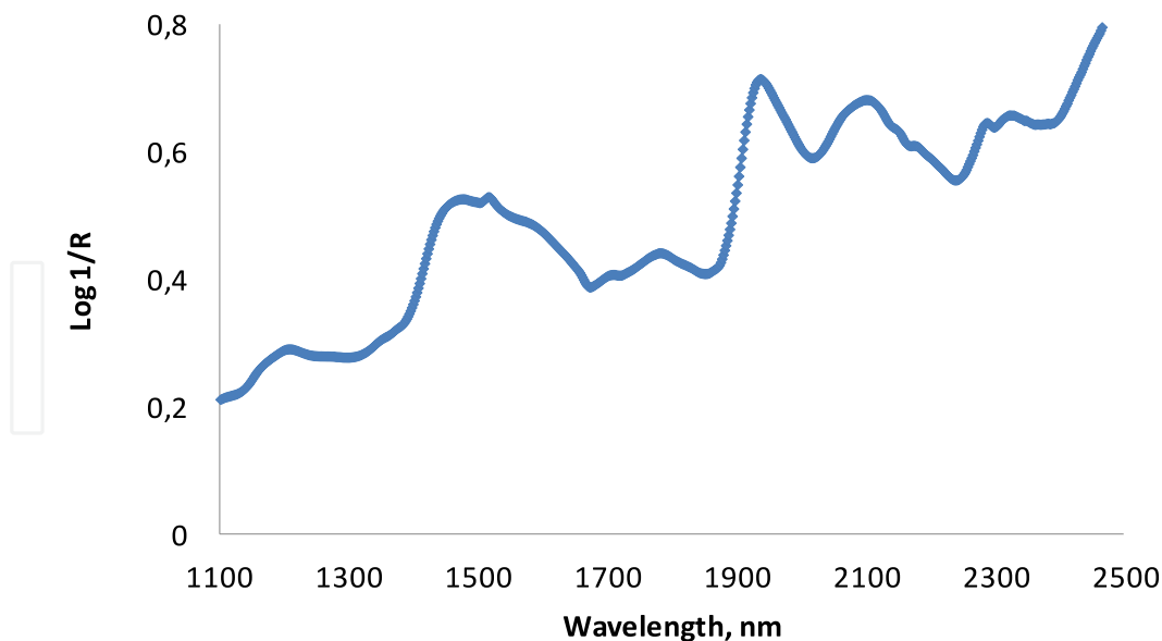
Fig. 1. NIR reflectance spectrum of wheat flour (1100-2500 nm) recorded by FOSS's NIRSystem 6500
