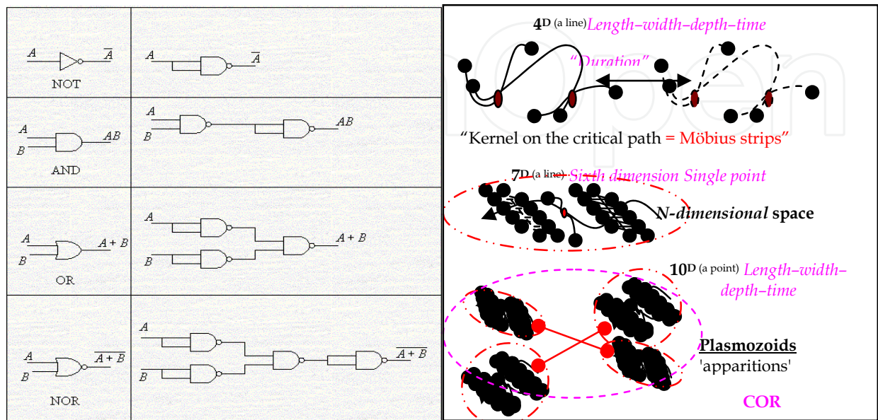
Fig. 9. N AND Equivalent Circuits Concept of WOSSI (COR gates) Logic circuit for function AB = AB i.e. the complement of "A NAND B" (Collins, 2002; Als, 1999).
