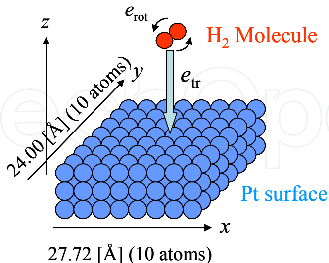
Fig. 4. Schematic diagram of simulation system.
