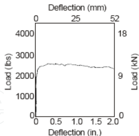
Fig. 11. Post-stabilization and before passing traffic results
