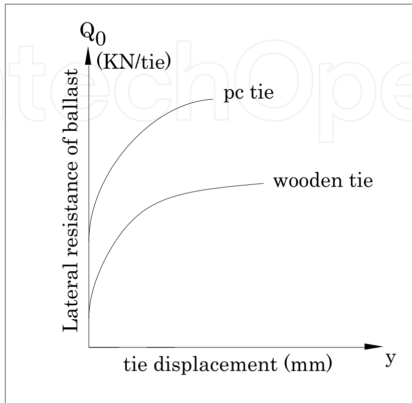
Fig. 3. The relationship between lateral resistances and displacement
